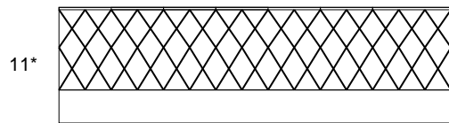
PL09 - Beachy Head
