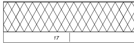
PL05 - Southwold
