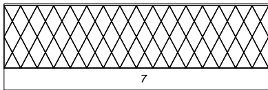
PL02 - Orford Ness
