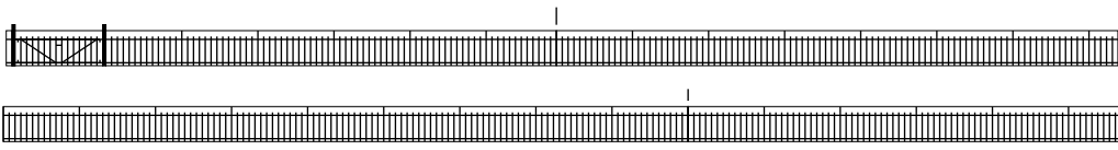
PL22 - Berry Head
