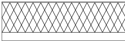
PL08 - Lowestoft
