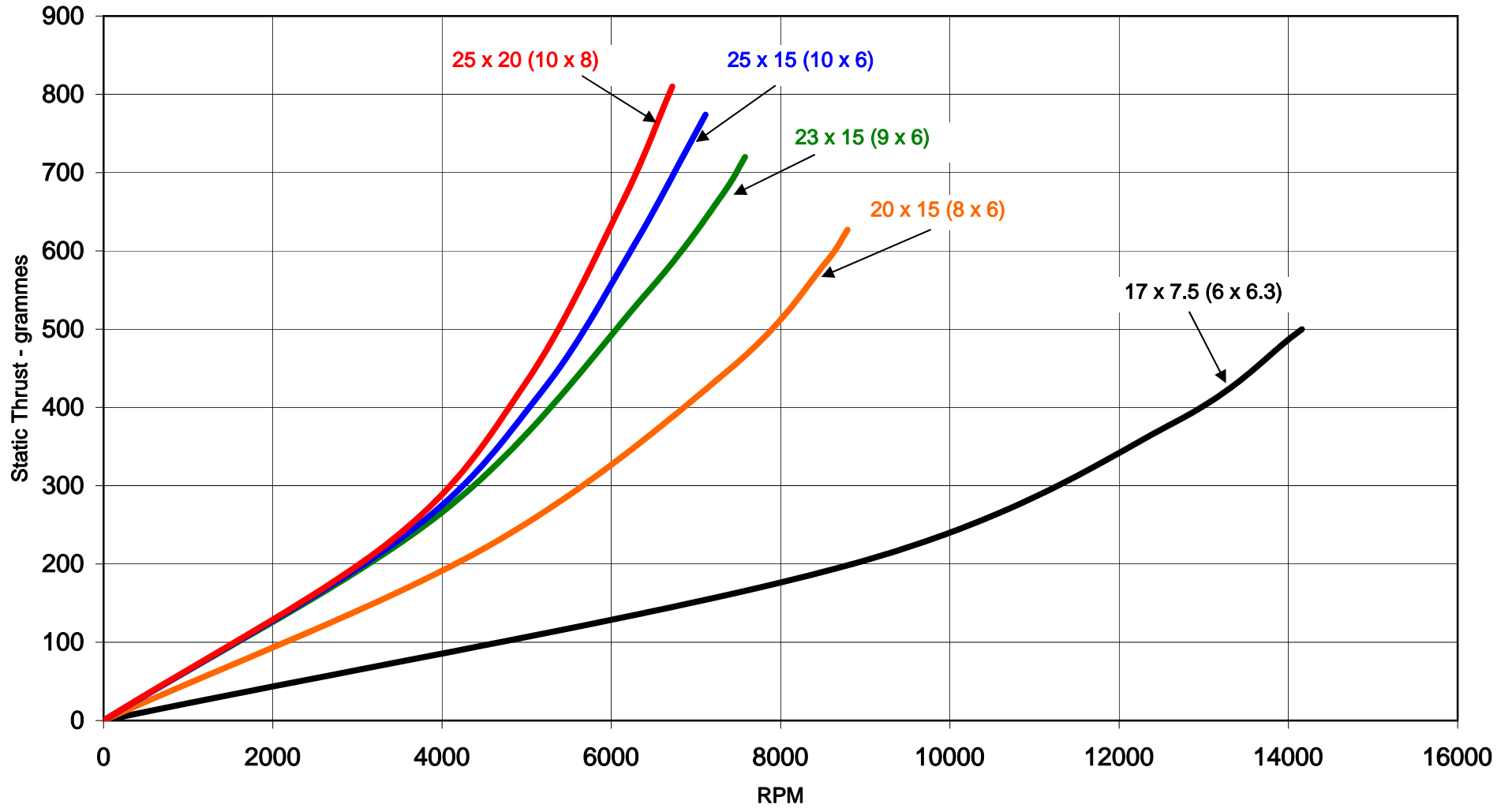
Graph 9 - Static Thrust curves for Graupner CAM SlimProps - Fixed blade.
