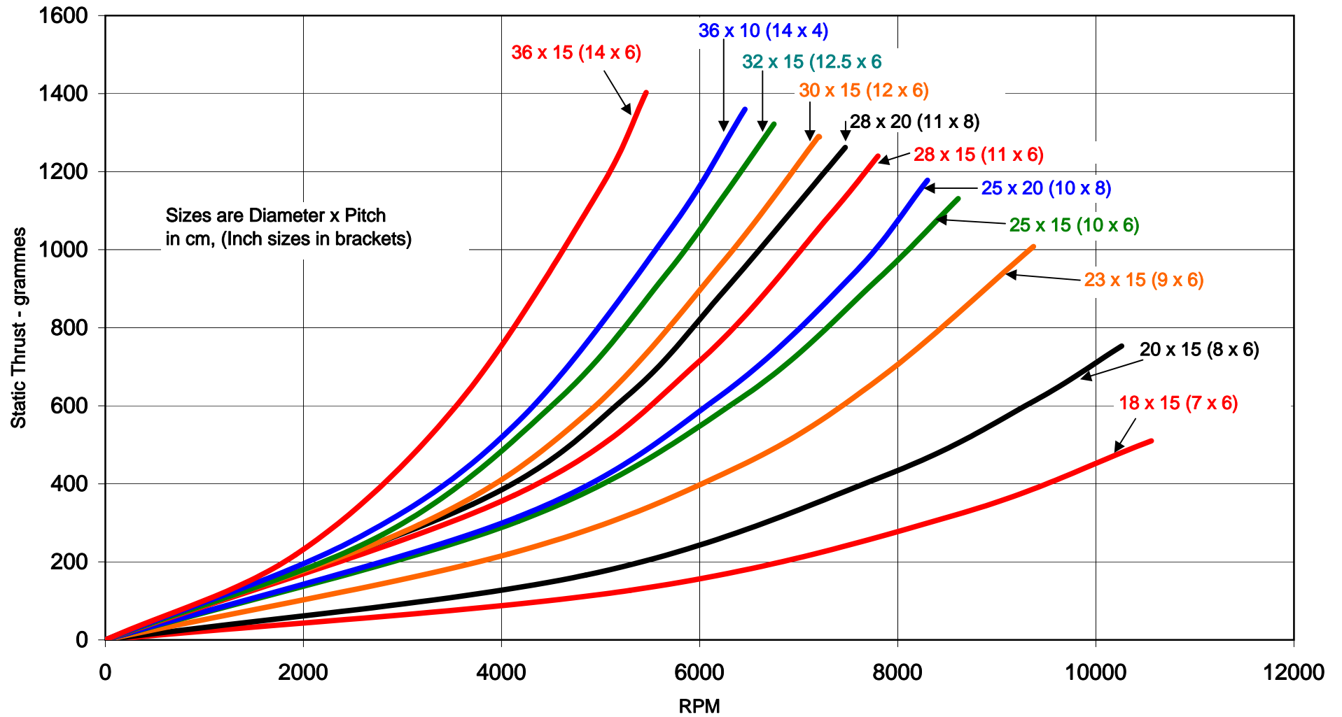
Graph 8 - Static Thrust curves for Graupner CAM Props - Fixed blade.
