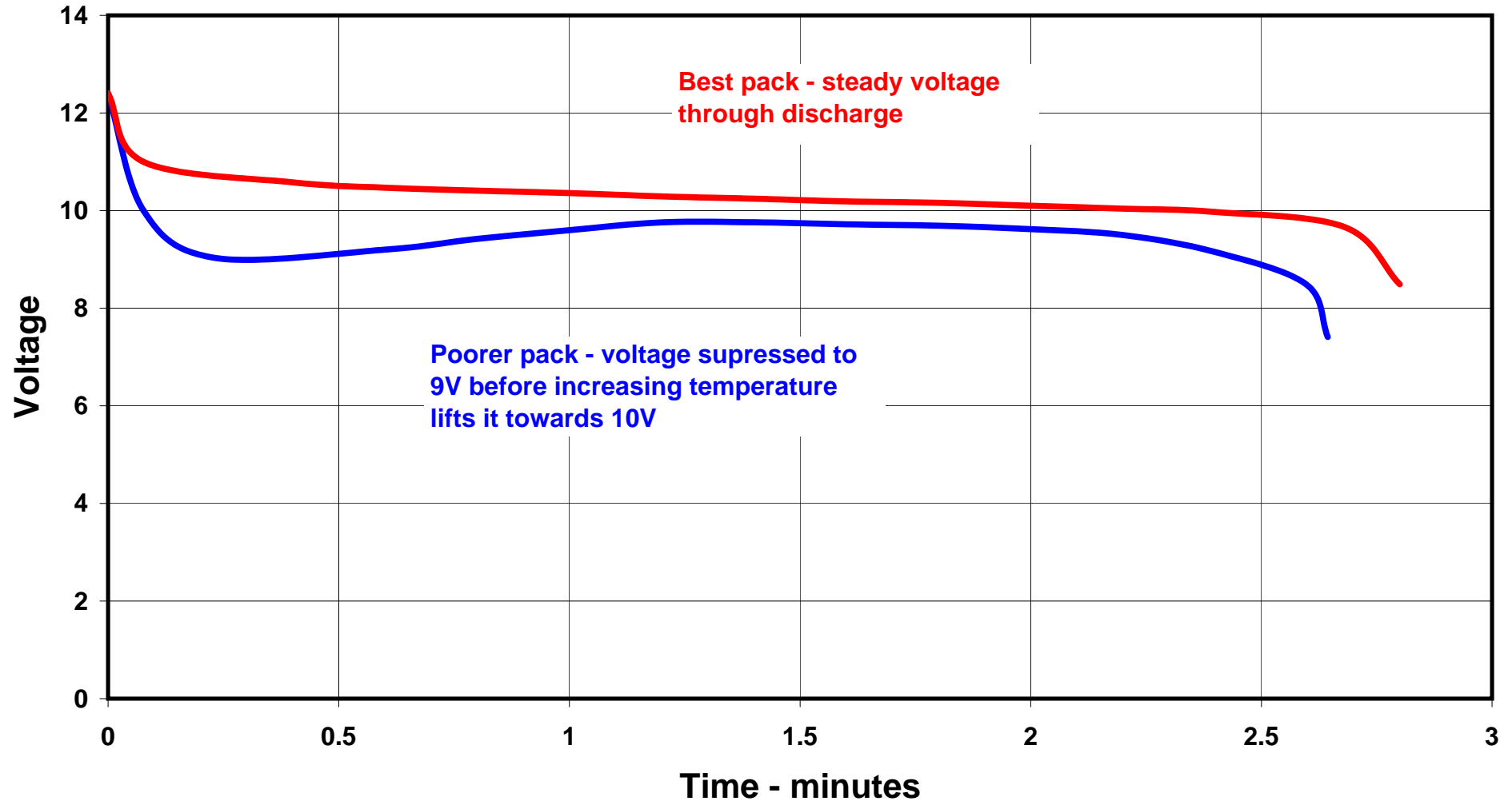
Graph 7 - 3S LiPos discharged at 20C showing voltage suppression
