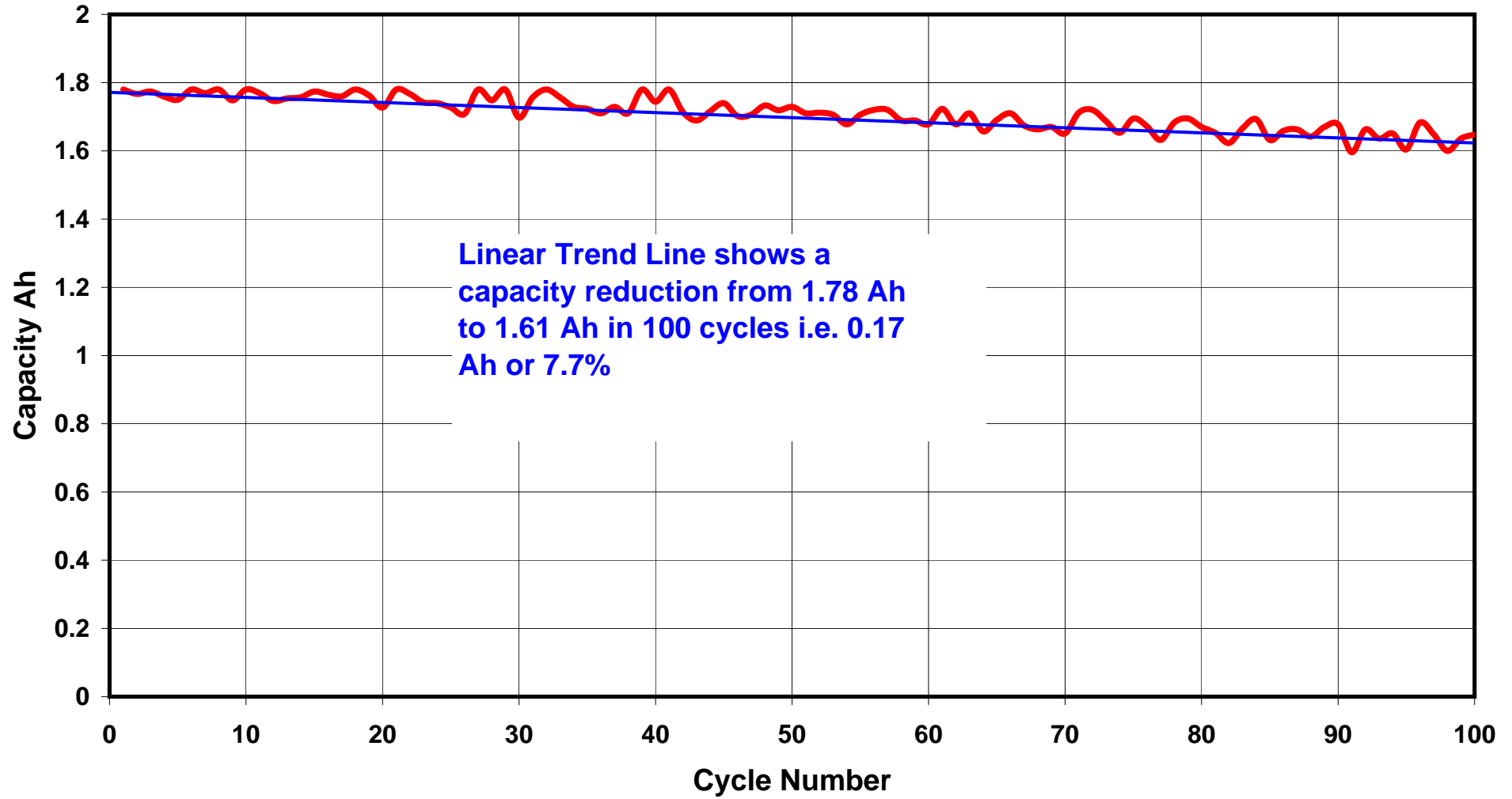
Graph 3 - Cyclic Capacity - HiModel 2200mAh 3S discharged at 44 amps (20C)
