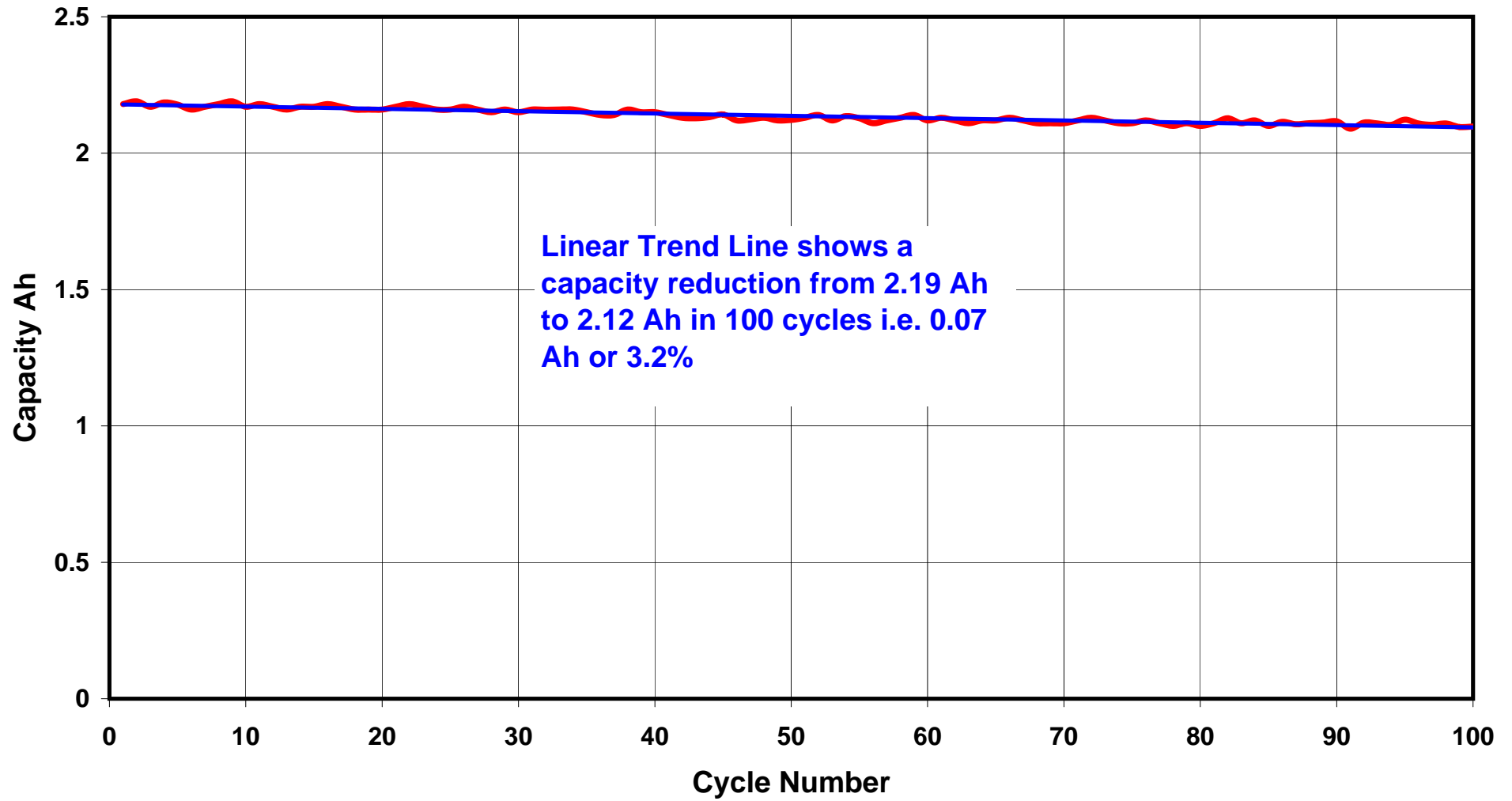
Graph 2 - Cyclic Capacity - Overtec Tornado 2200mAh discharged at 44 amps (20C)
