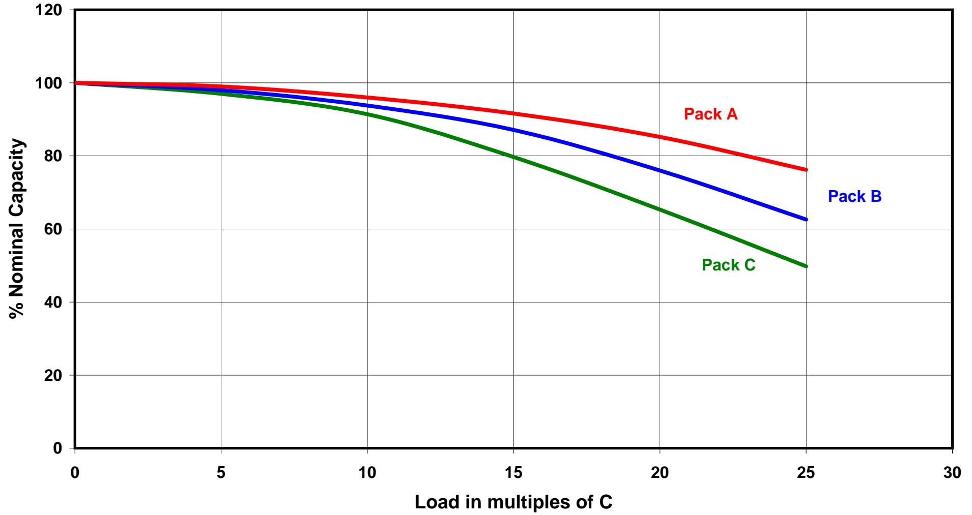
Graph 6 - Capacity loss with increasing load.
