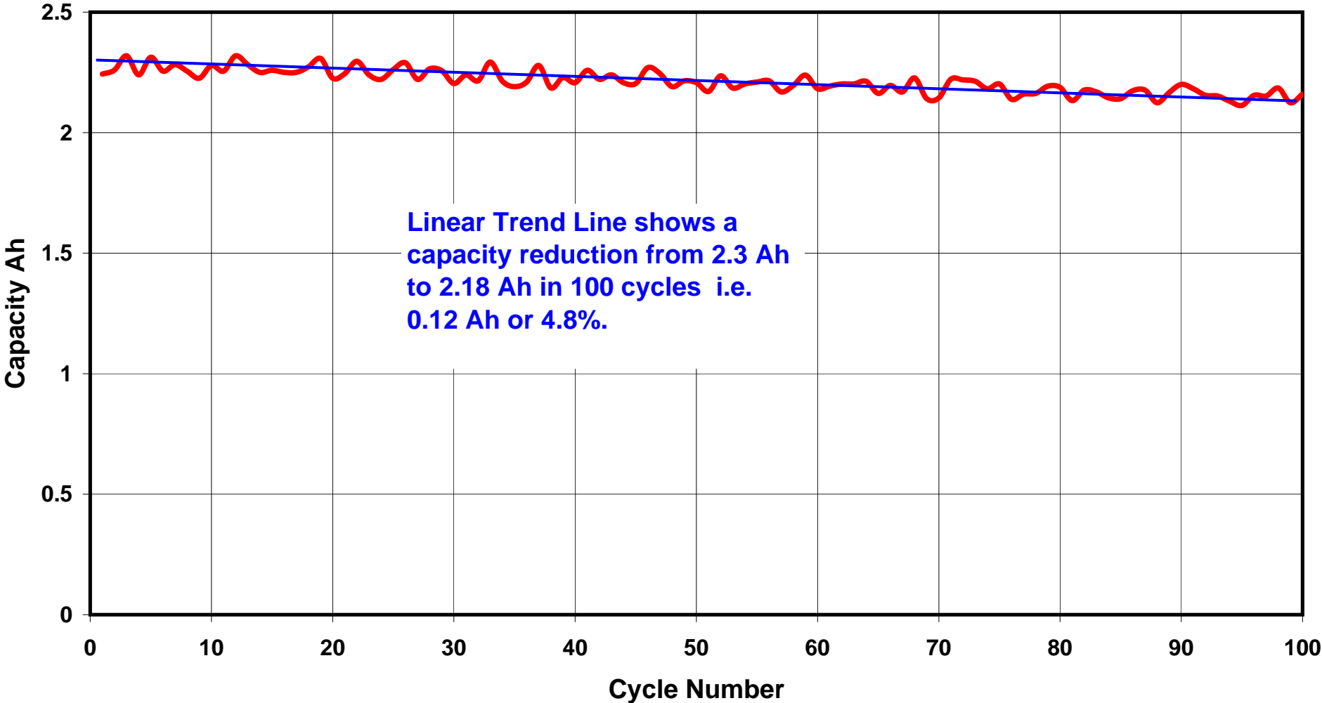
Graph 5 - Cyclic Capacity - Electrolite 2500mAh 3S discharged at 50 amps (20C).
