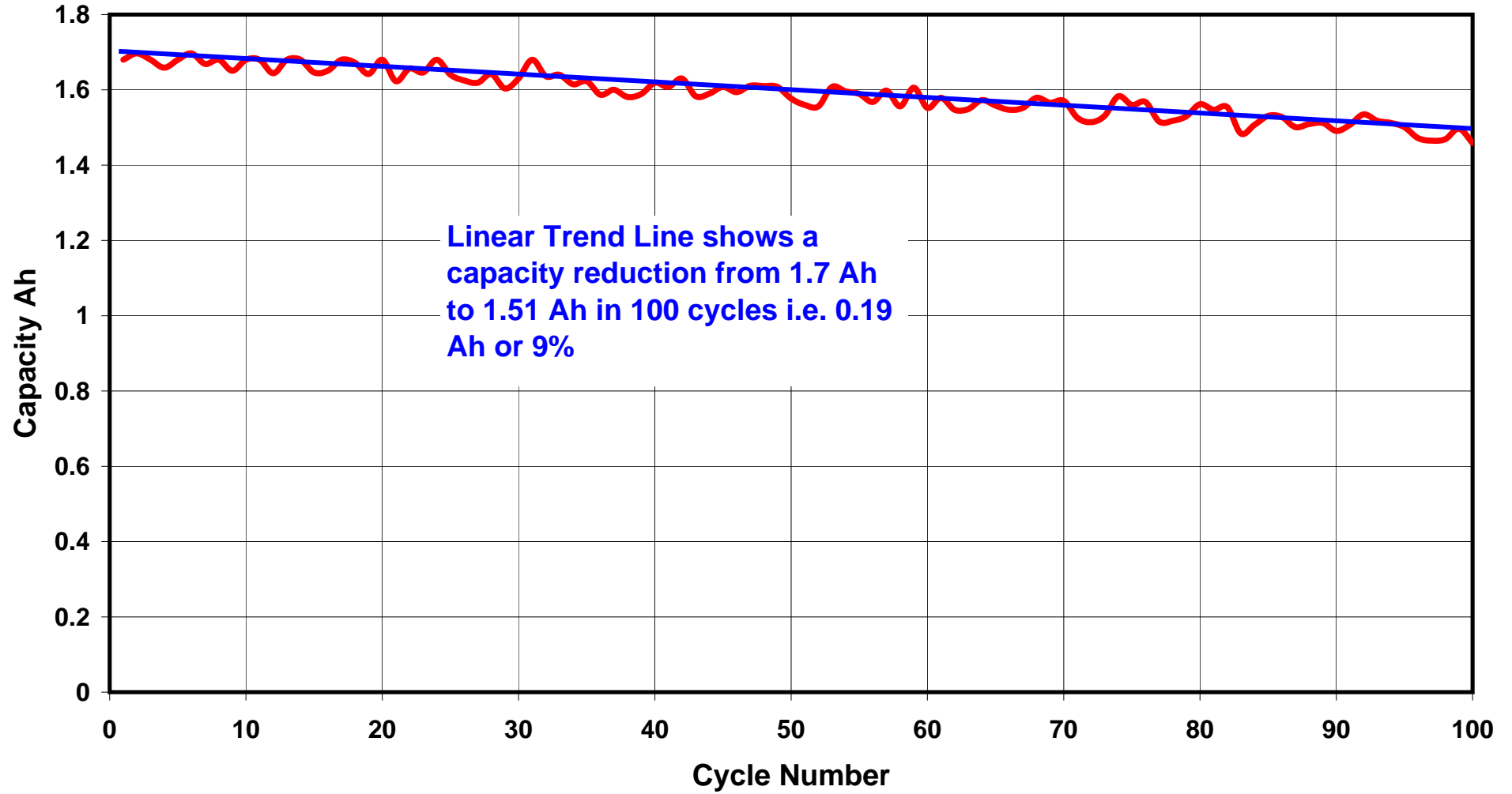
Graph 4 - Cyclic Capacity - ModelPower 2150mAh 3S discharged at 43 amps (20C)
