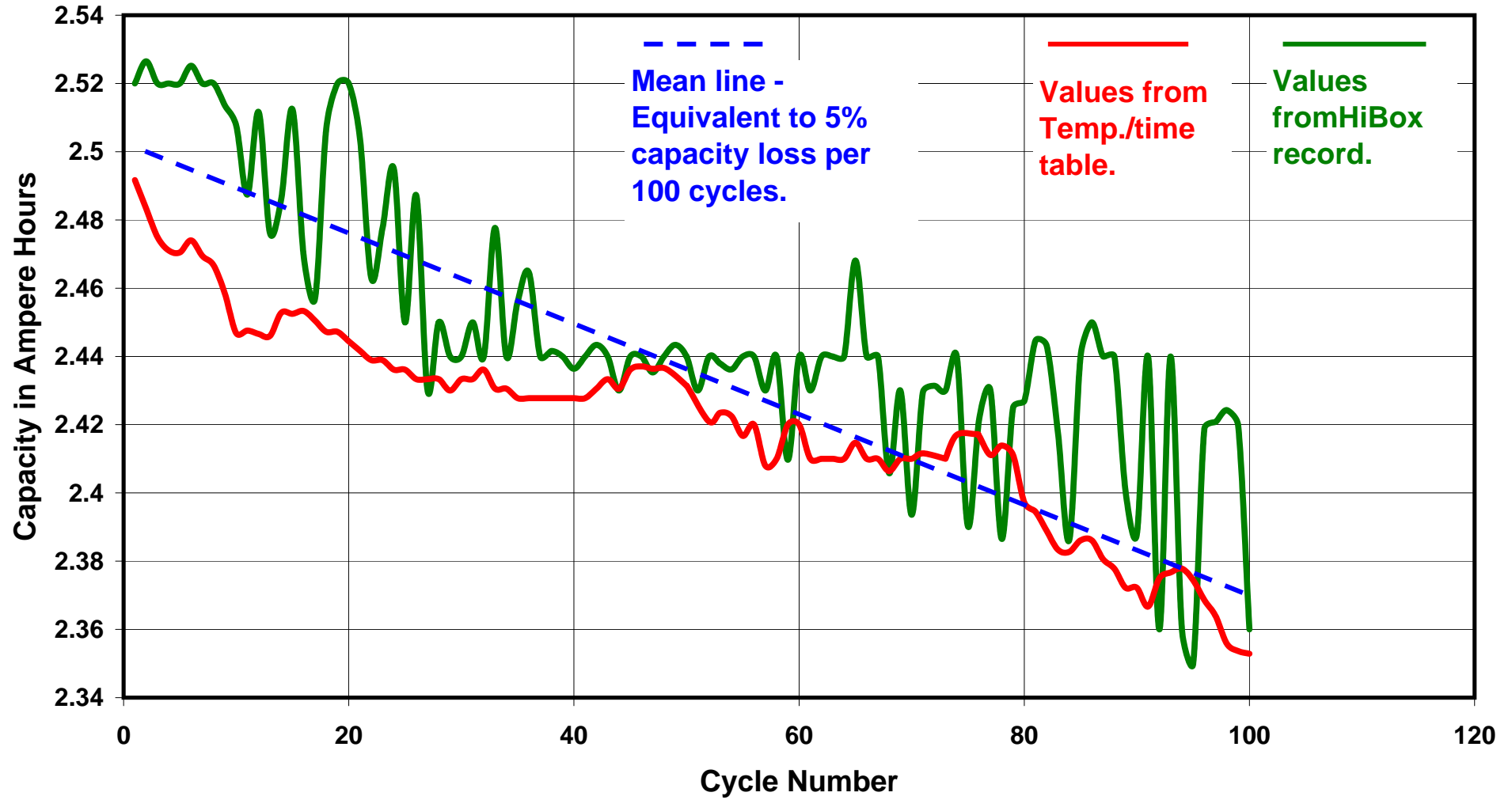
Graph 1 - Capacity Reduction for 3C Discharge cycle
