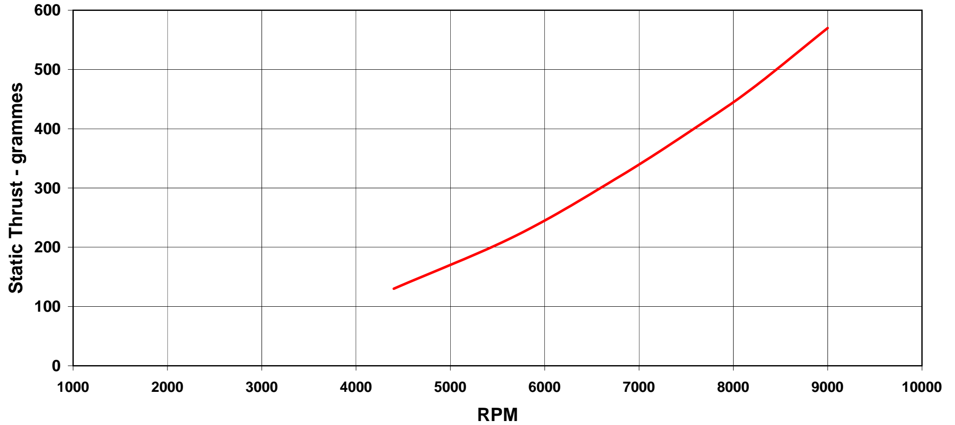
Graph 2 - Propeller Calibration - GWS 8" x 4.3"
