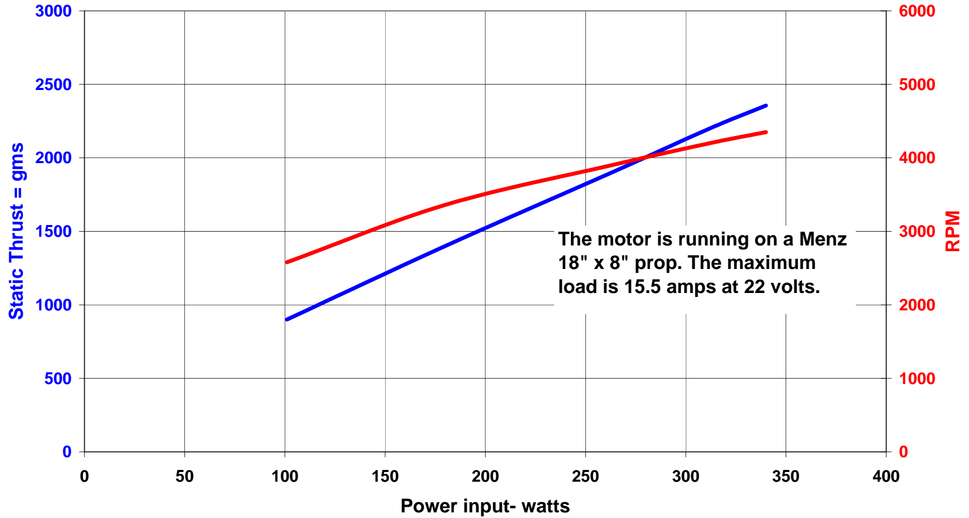
Graph 3 -The Hacker A60 - 14L on a 6 cell 3200 mAh LiPo pack
