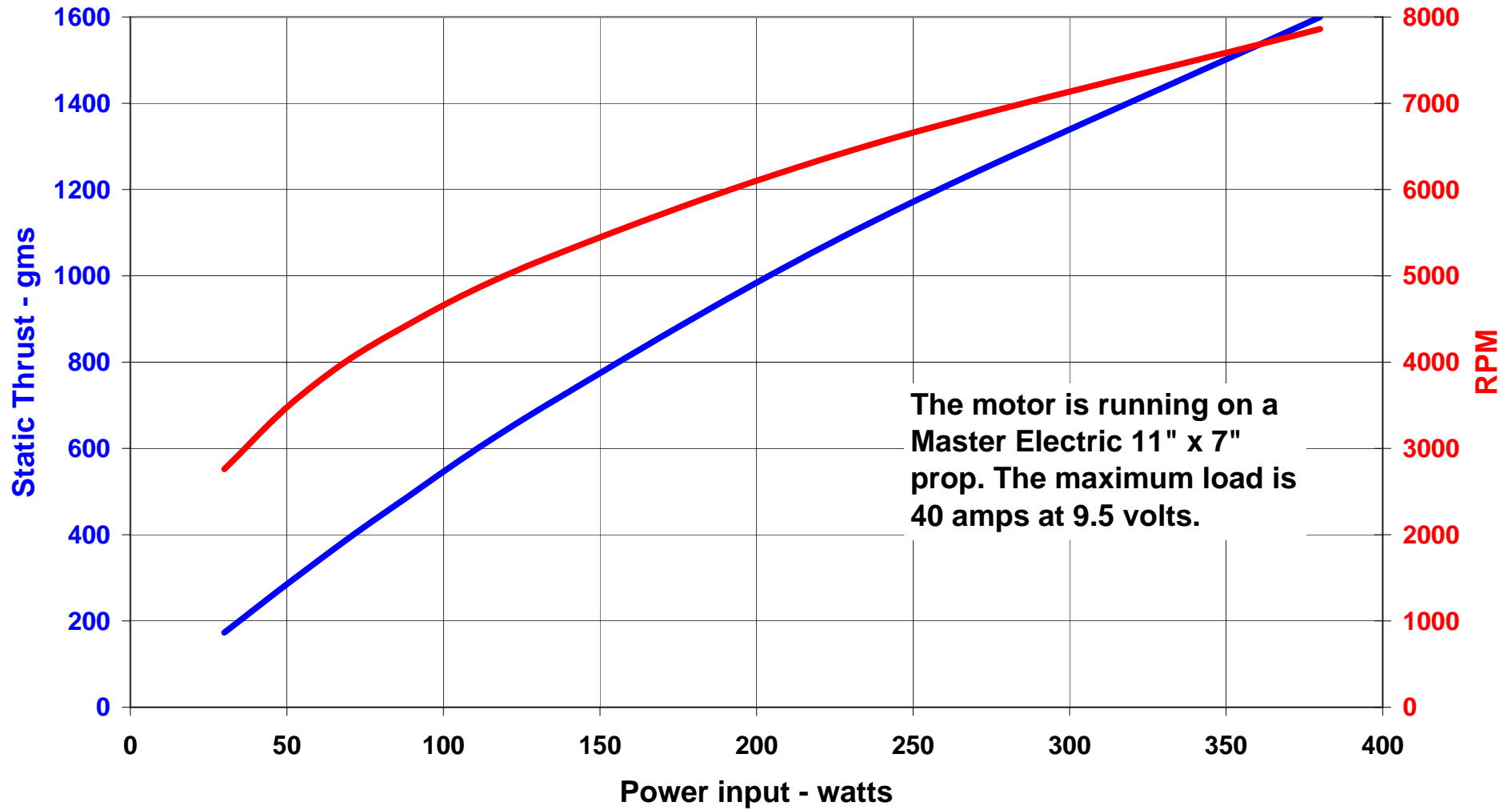
Graph 1 - The Hacker A30-8XL on a 3 cell 3200 mAh LiPo pack
