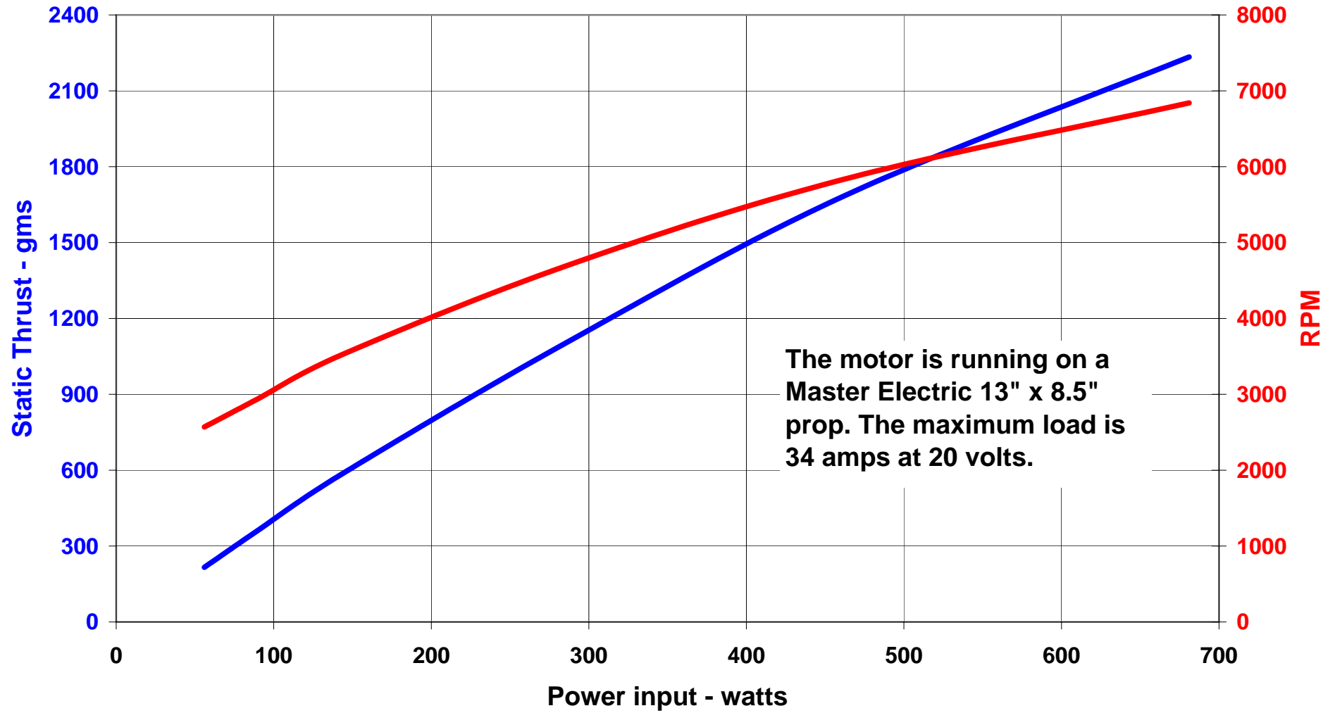
Graph 2 - The Hacker A50-10S on a 6 cell 3200 mAh LiPo pack
