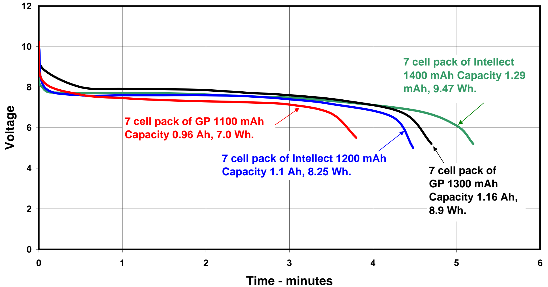
Graph 1 - Discharge of 2/3 A sized cells at 15 amps
