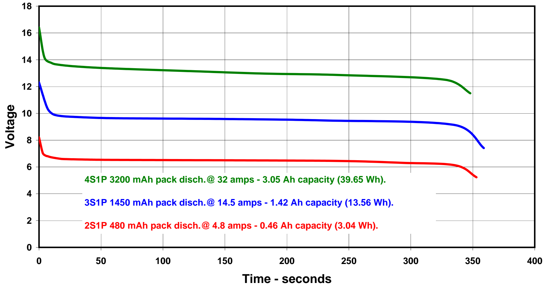
Graph 2 - Discharge of Impulse LiPos at 10C rating.
