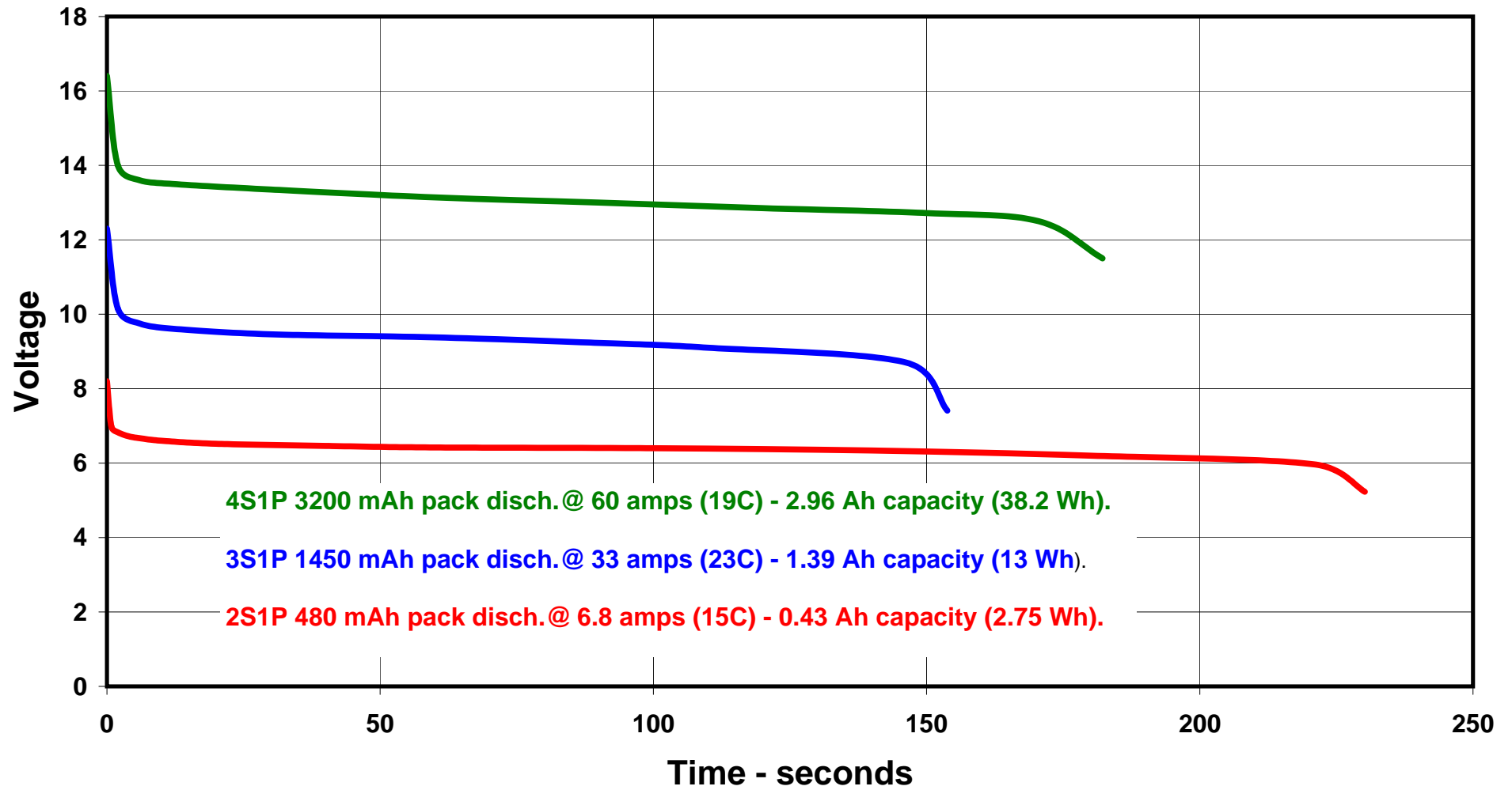
Graph 3 - Discharge of Impulse LiPos at max. rating.
