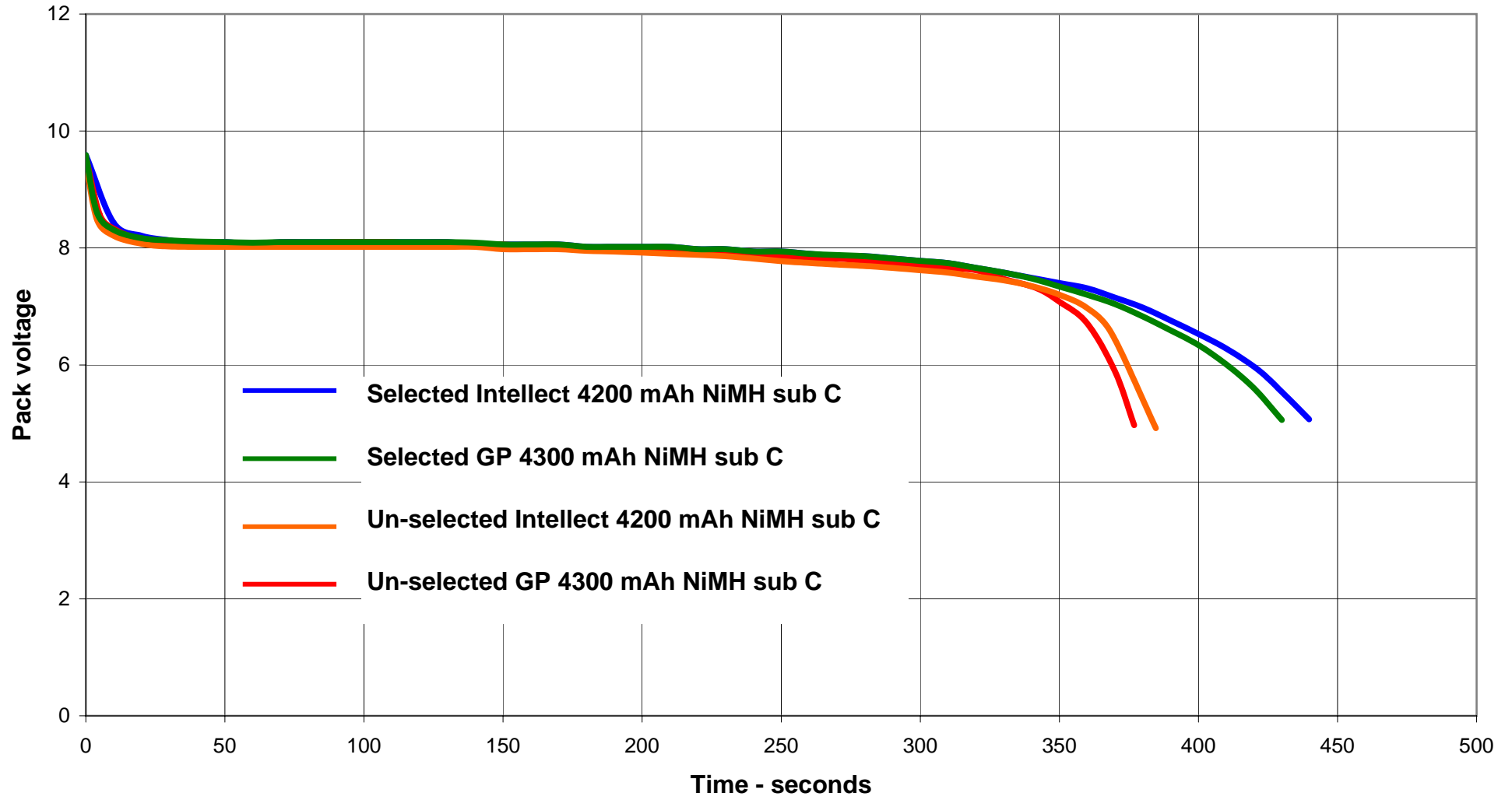
Graph 1 - Discharge for four 7 cell packs.
