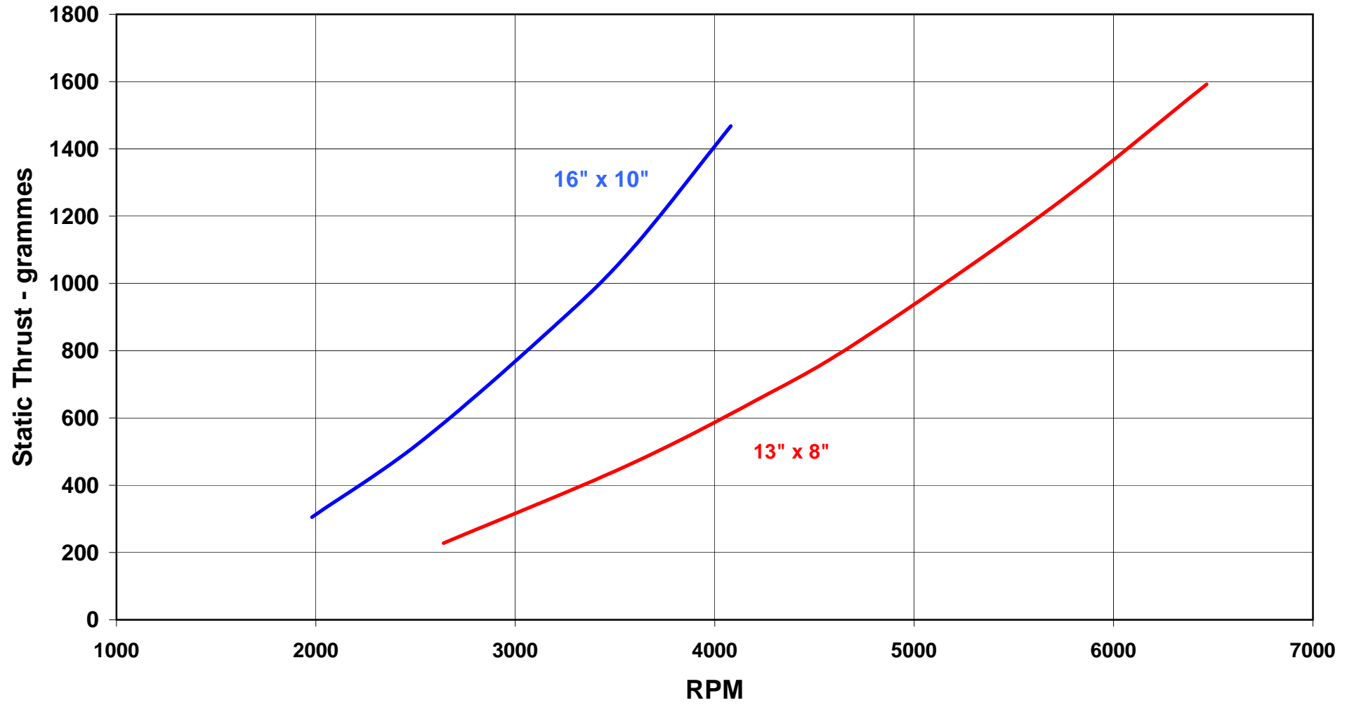
Graph 1 - Propeller Calibration - Aeronaut Cam Folders
