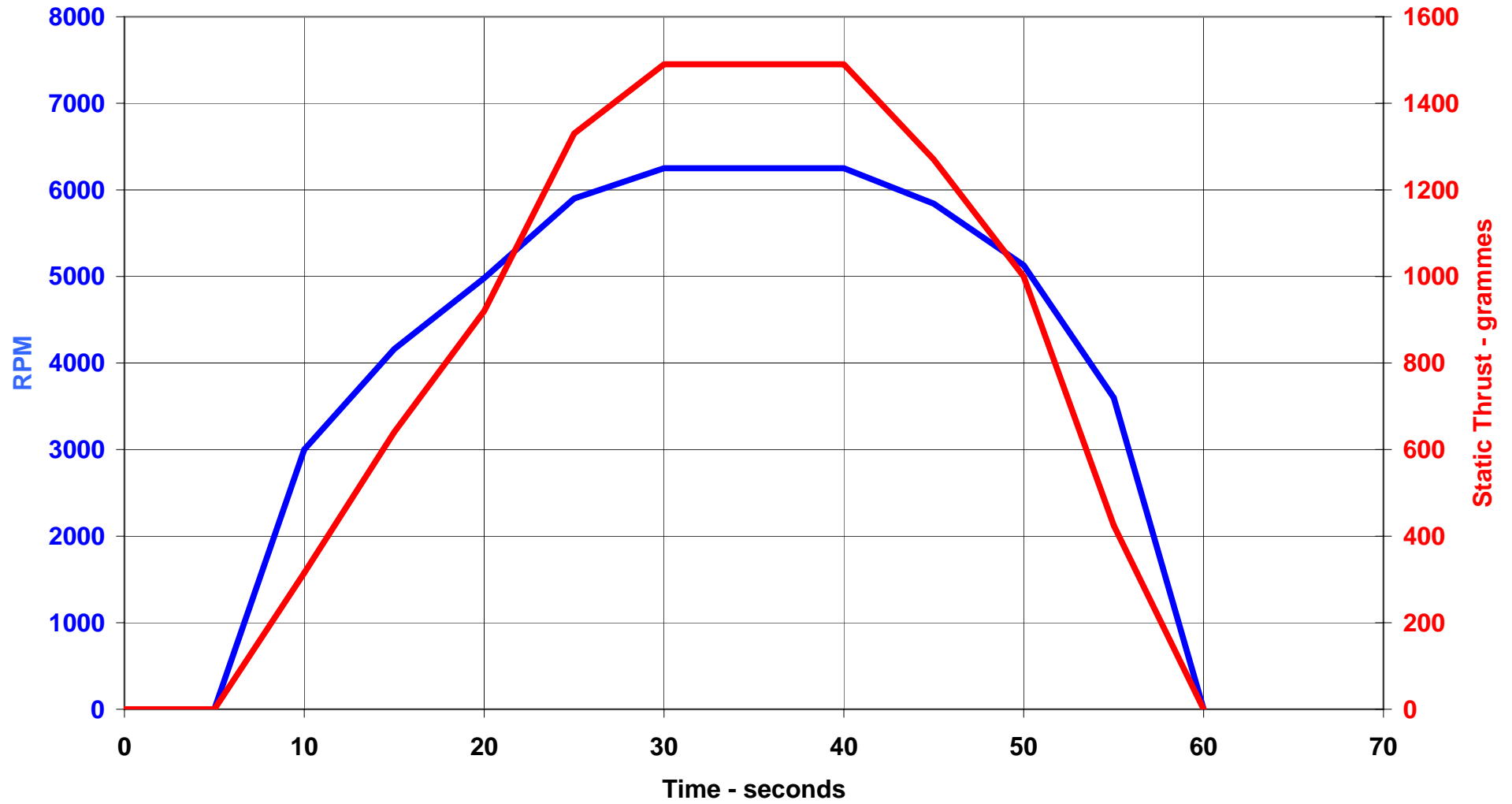
Graph 4 - Conversion of RPM values to Static Thrust.
