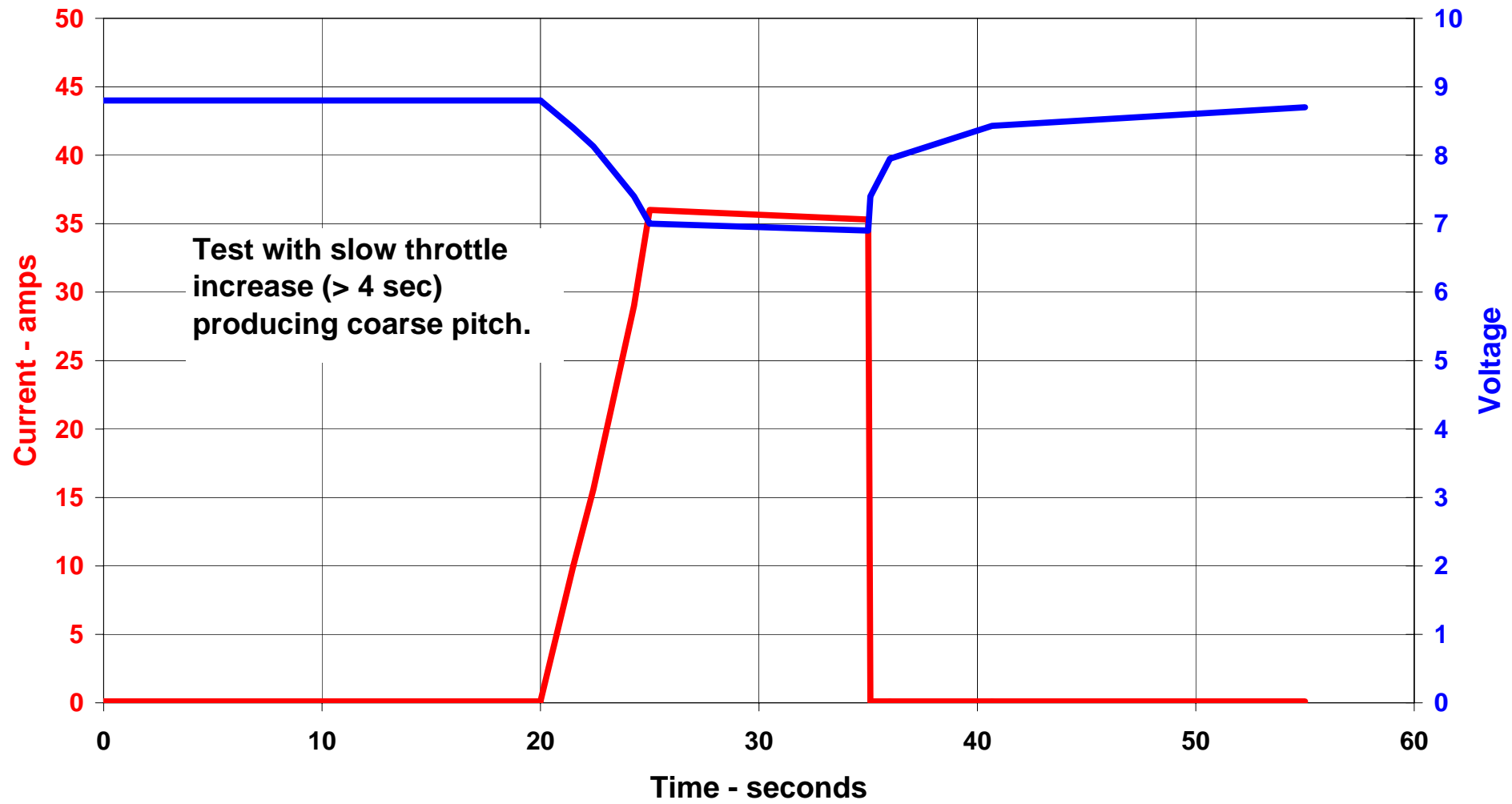
Graph 1 - Kavan 2 Pitch Hub Test
