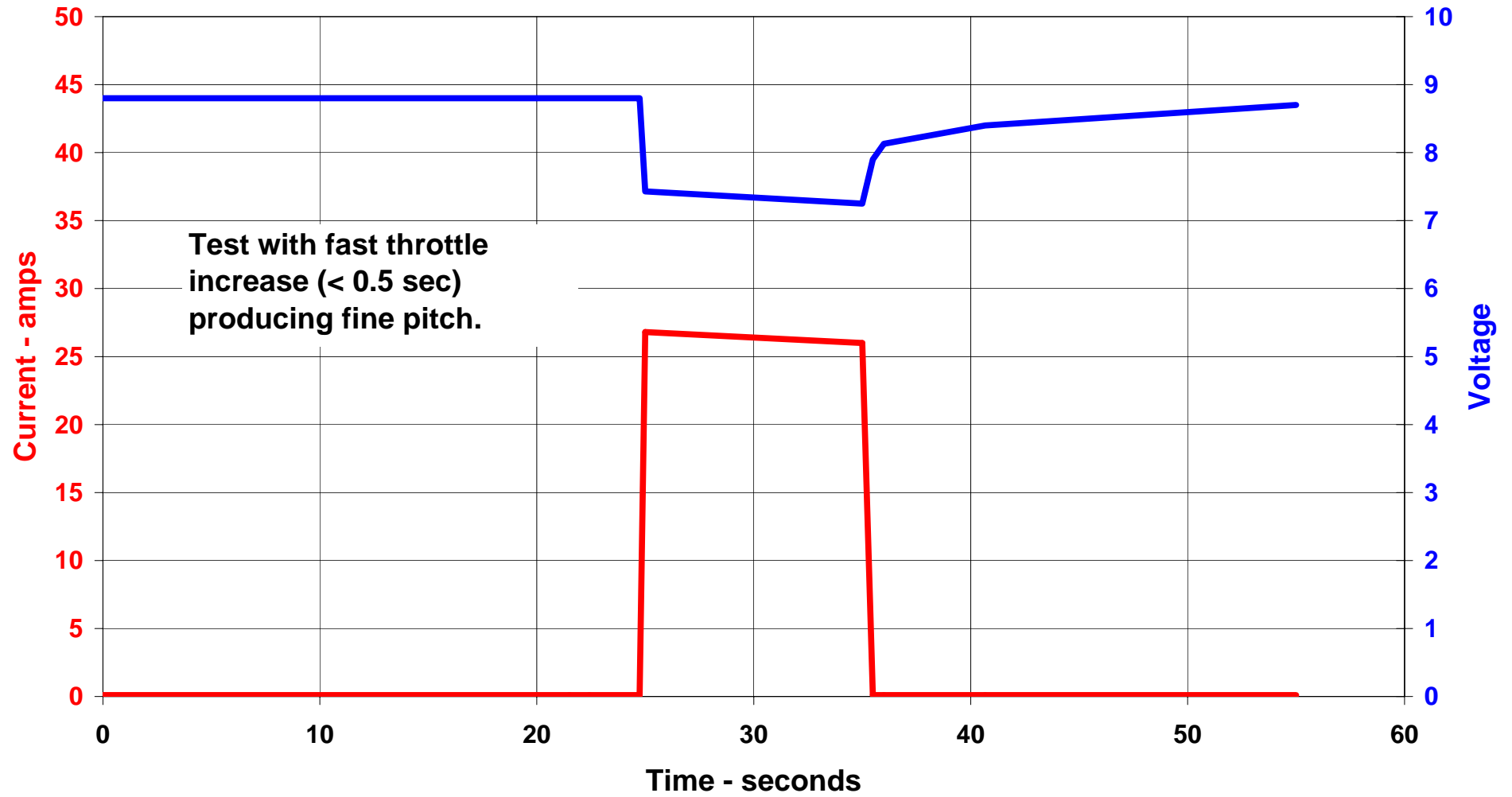
Graph 2 - Kavan 2 Pitch Hub Test
