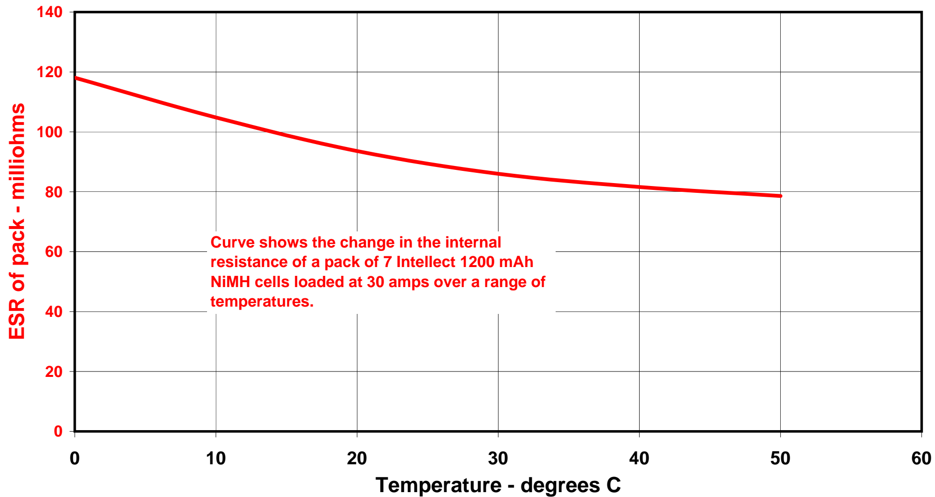
Graph 7 - ESR variation with temperature.
