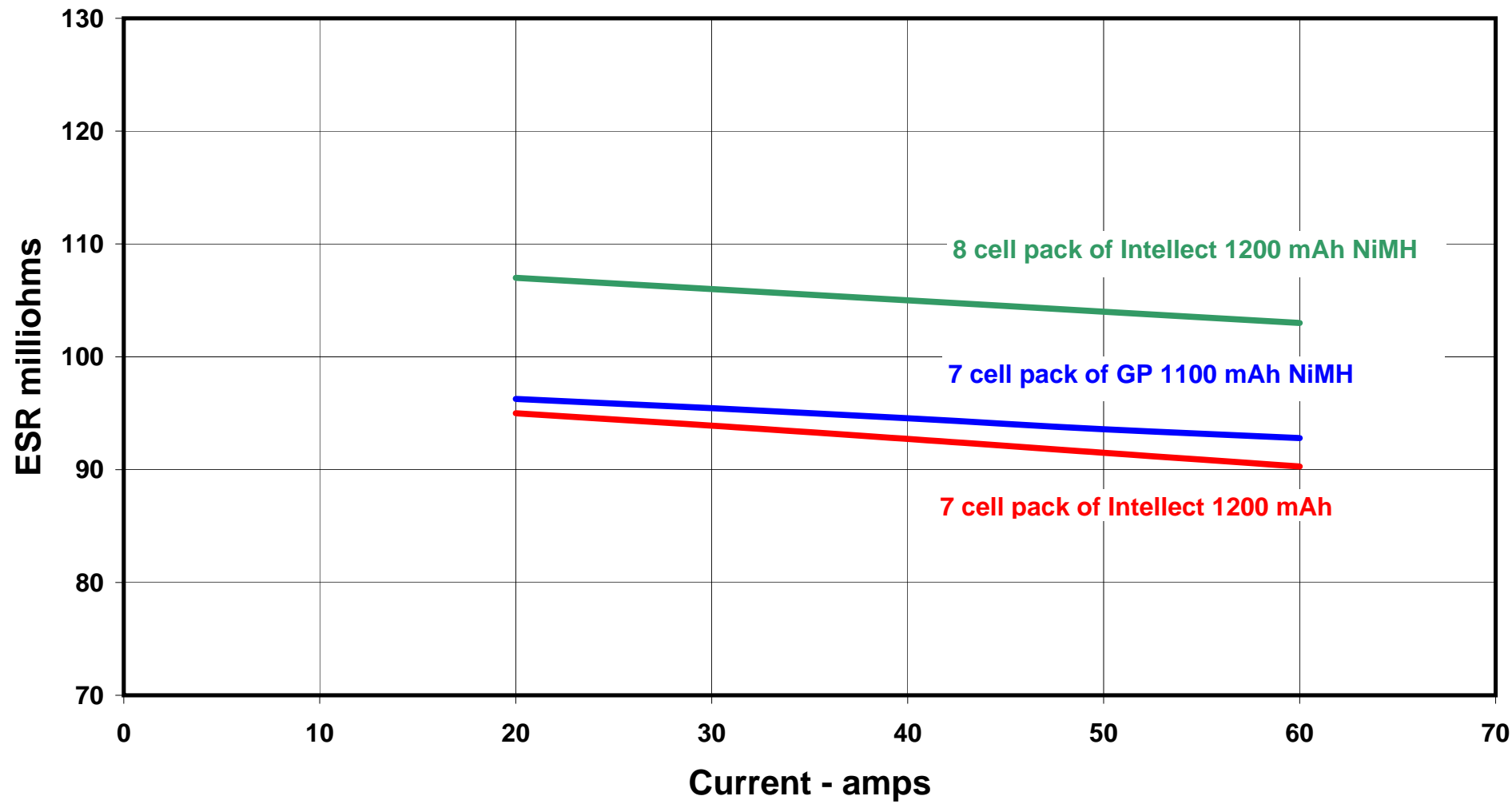
Graph 6 - Pack Internal Resistances
