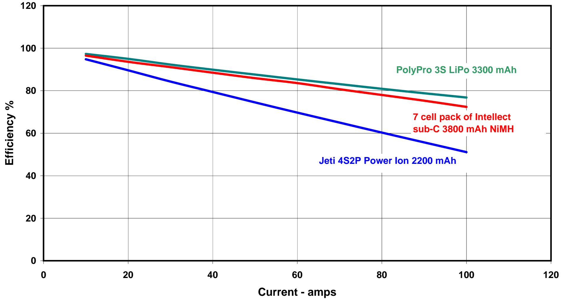
Graph 5 - Efficiency for different cell types.
