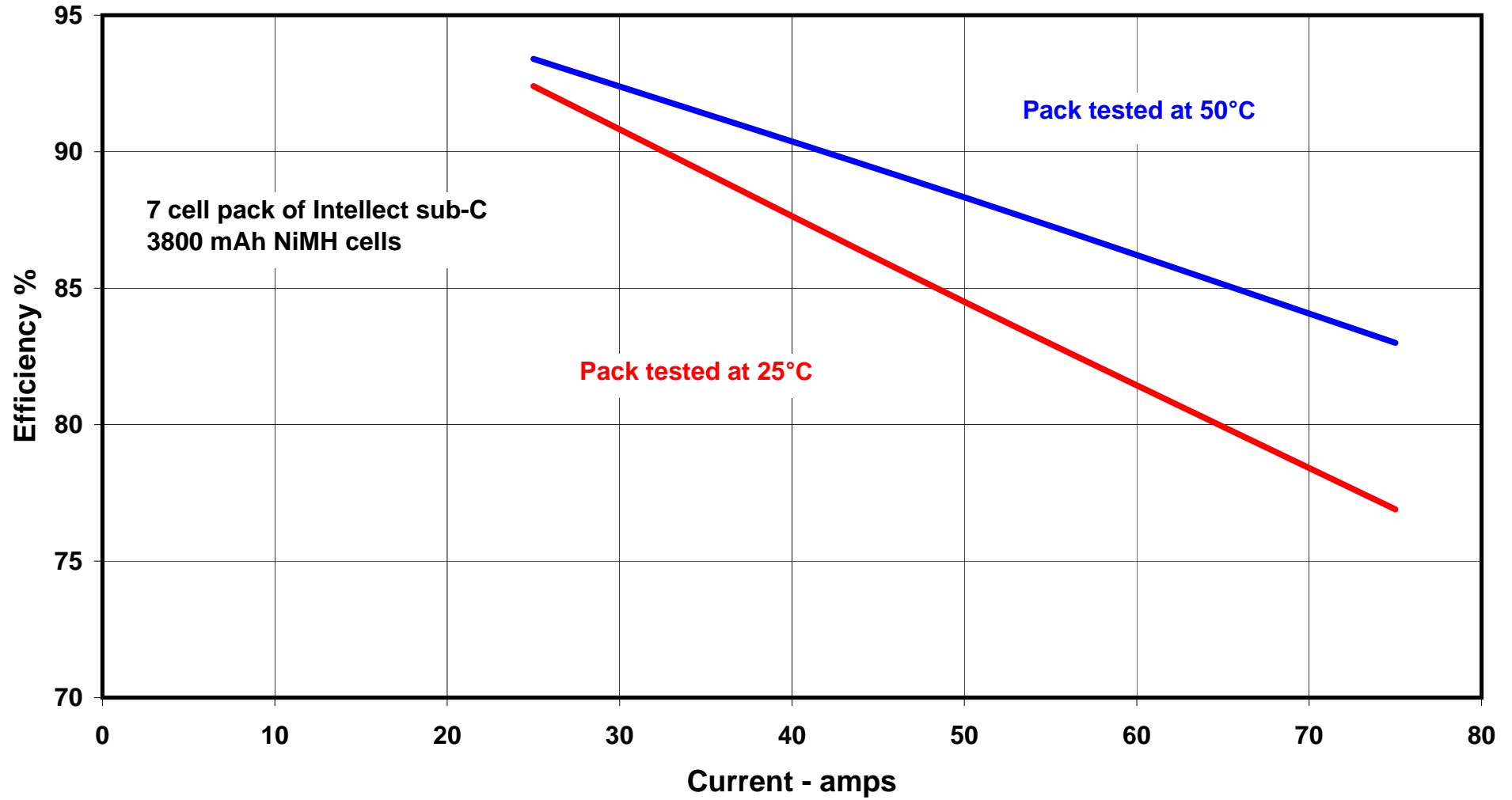
Graph 3 - Efficiency at varying temperature
