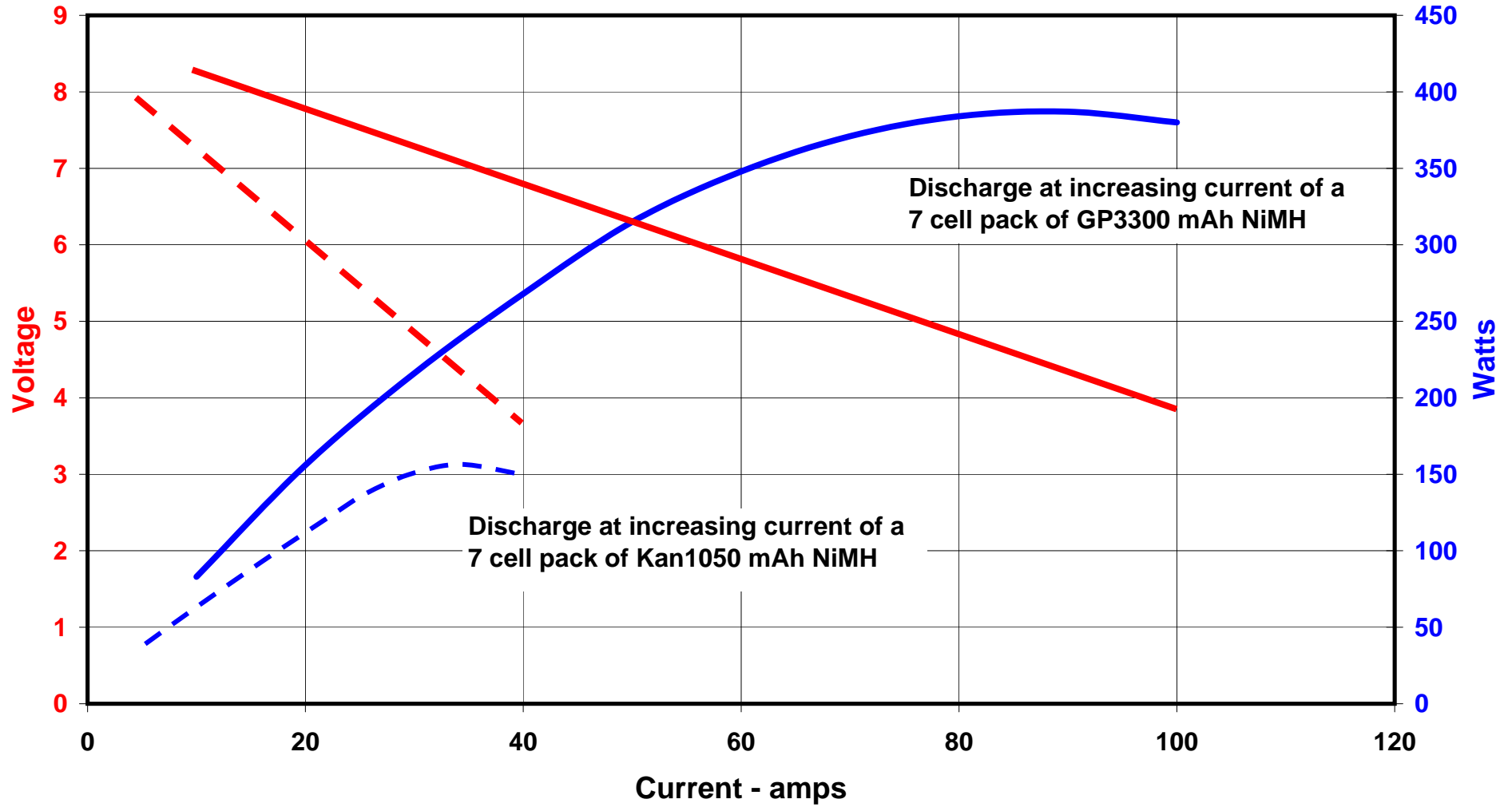
Graph 1 - Theoretical Voltage and Wattage against current
