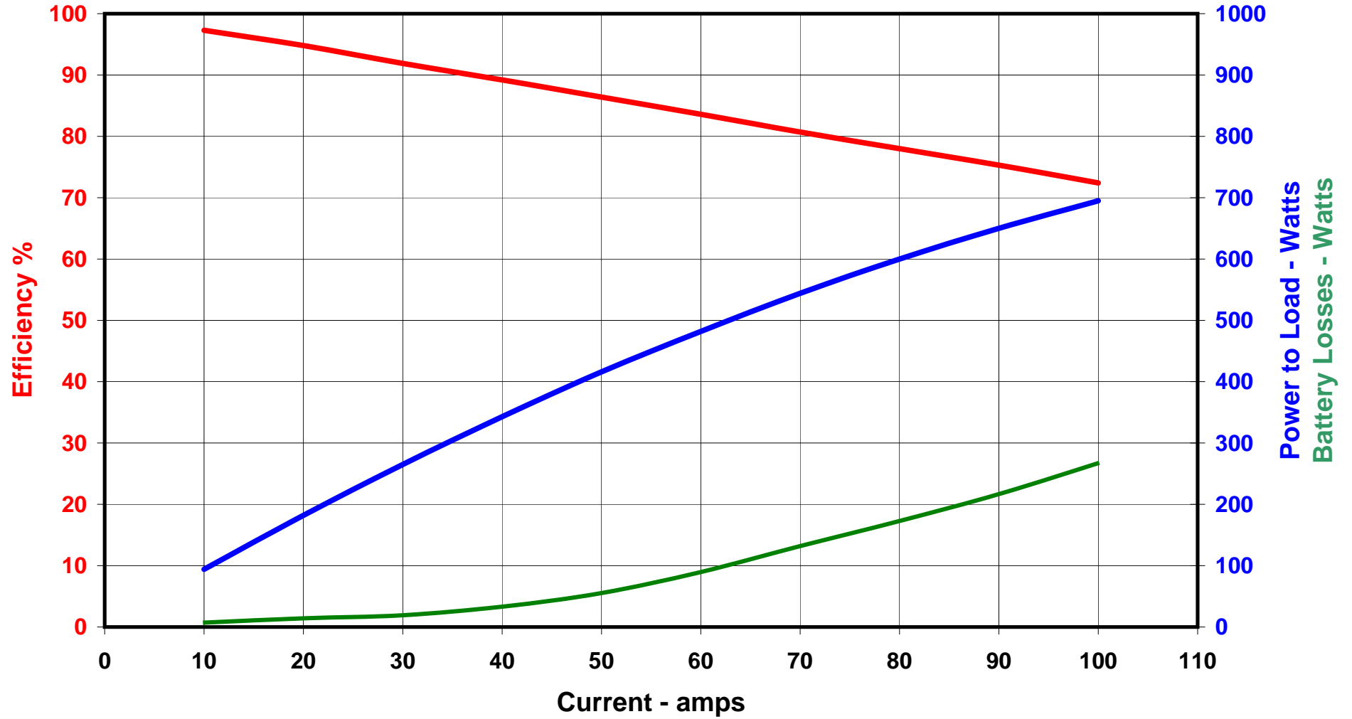
Graph 2 - 7 cell pack of Intellect 3800 mAh NiMH - full results (Pack Temperature 35°C)
