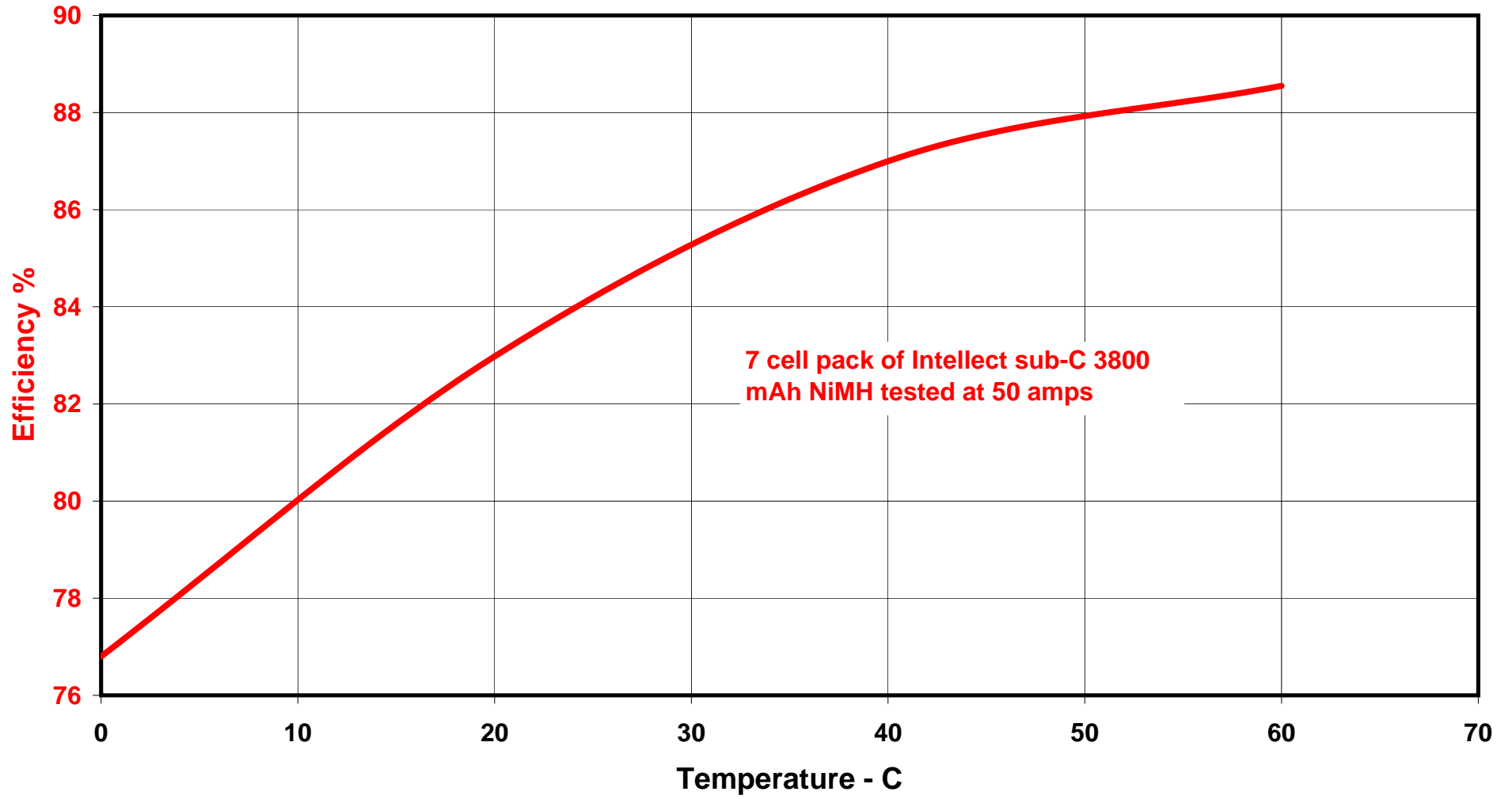
Graph 4 - Efficiency at increasing temperature
