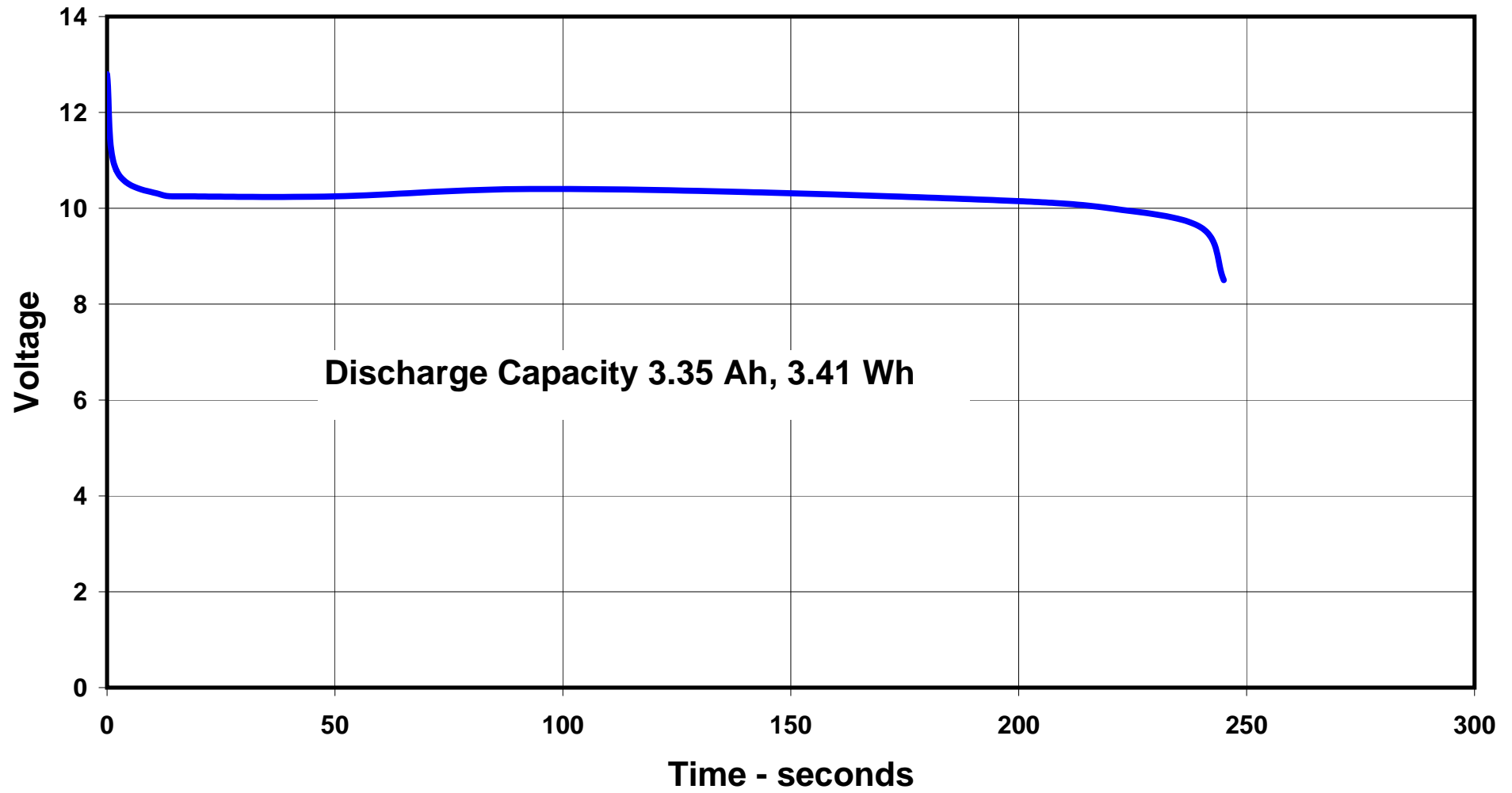
Graph 2 - Discharge of Overlander PolyPro 3300 3S pack at 50 amps/15C
