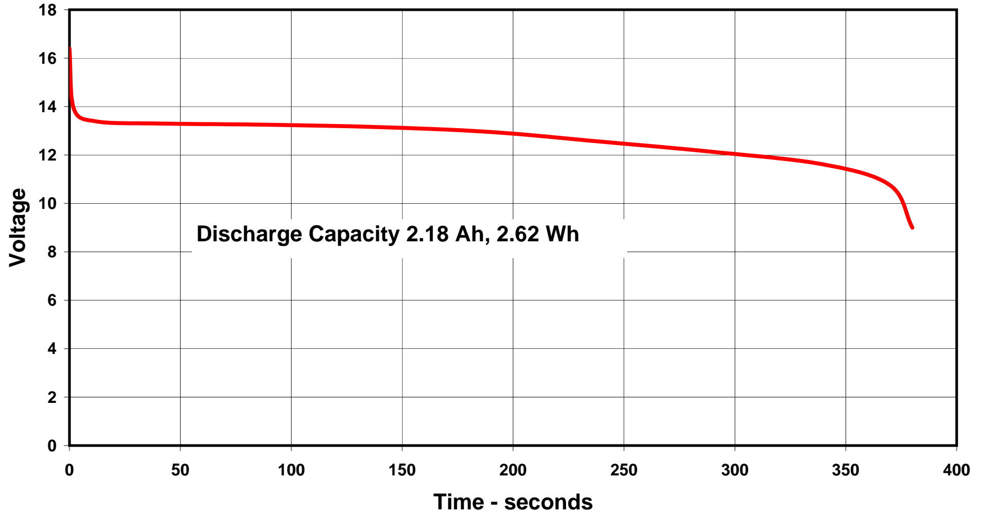
Graph 1 - Discharge of Jeti Power-Ion 4S2P at 20 amps/9C.
