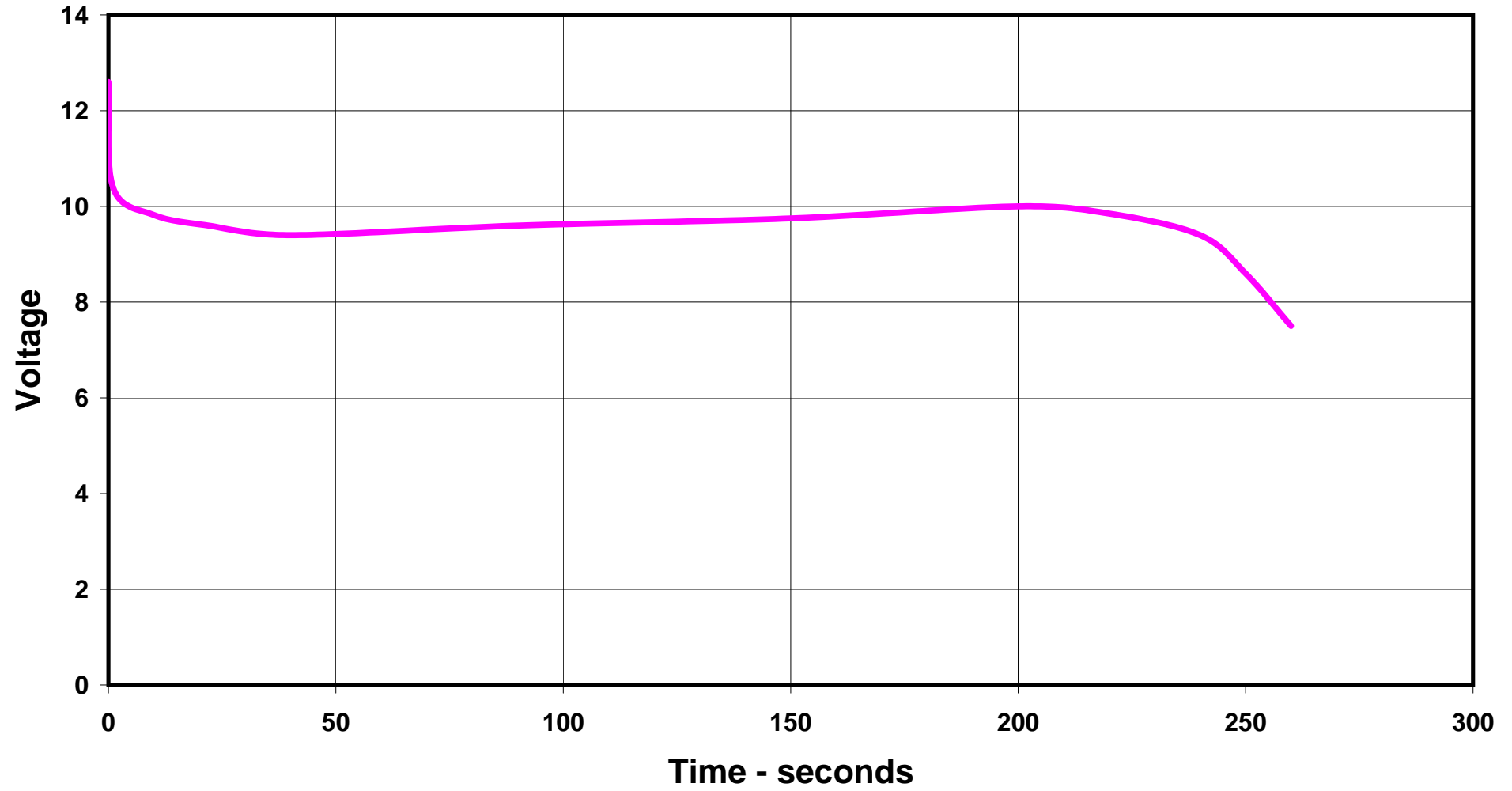
Graph 5 - Discharge of Thunder Power 1.3 Ah 3S LiPo pack at 16 amps/13C
