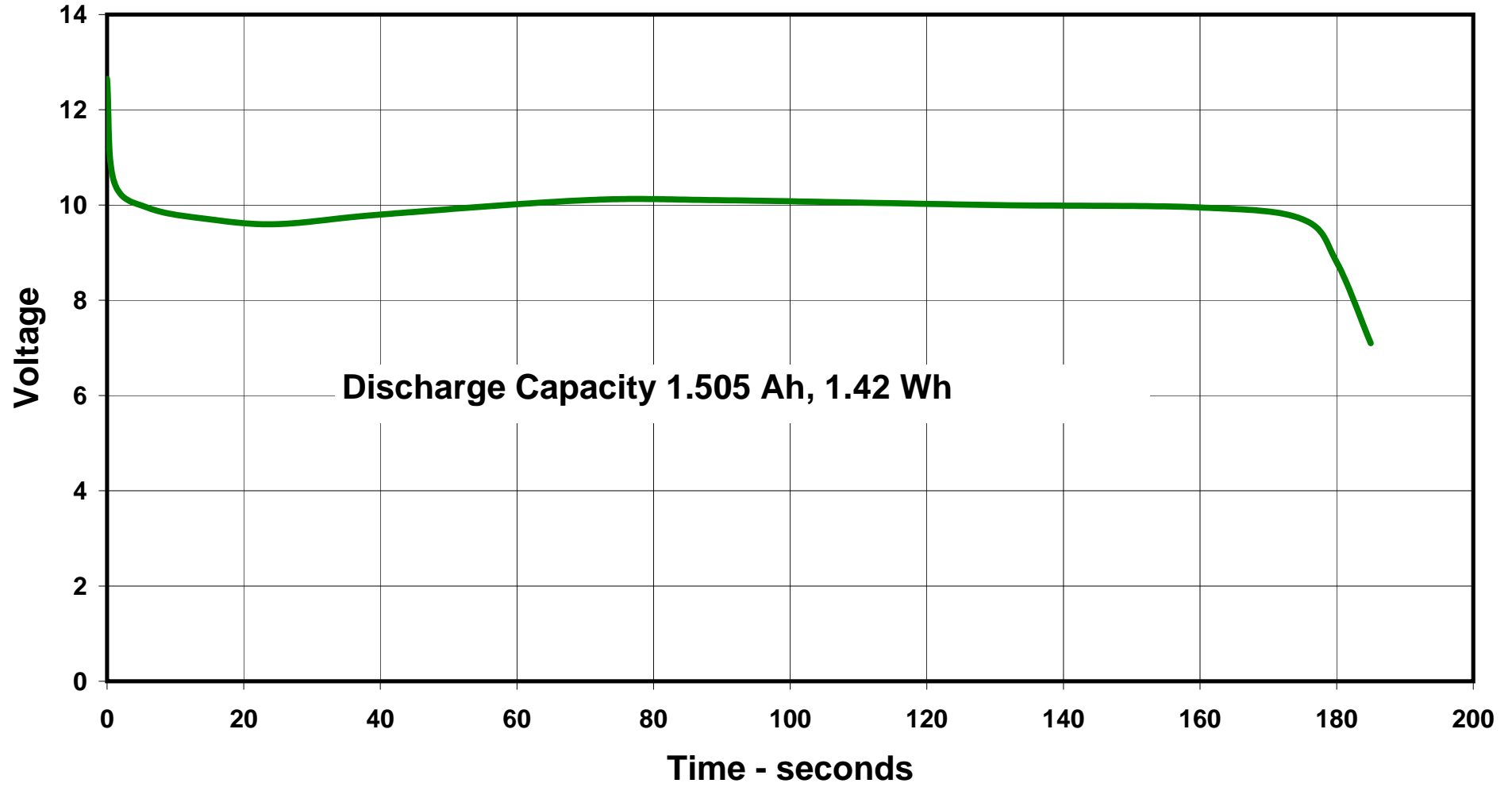
Graph 3 - Discharge of Overlander PolyPro 1500 3S pack at 30 amps/20C
