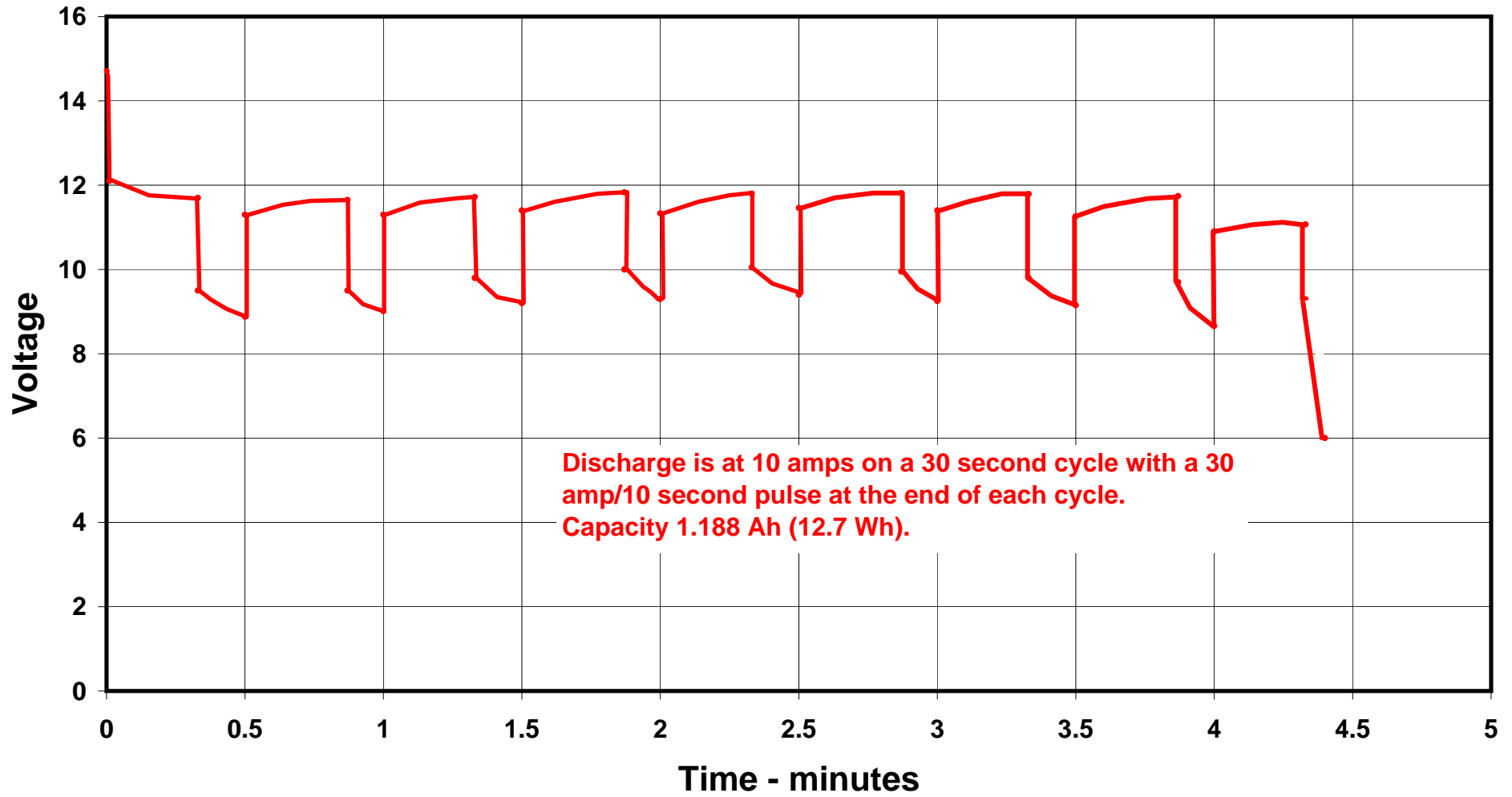
Graph 3 - Saphion 4S Pulse Discharge.
