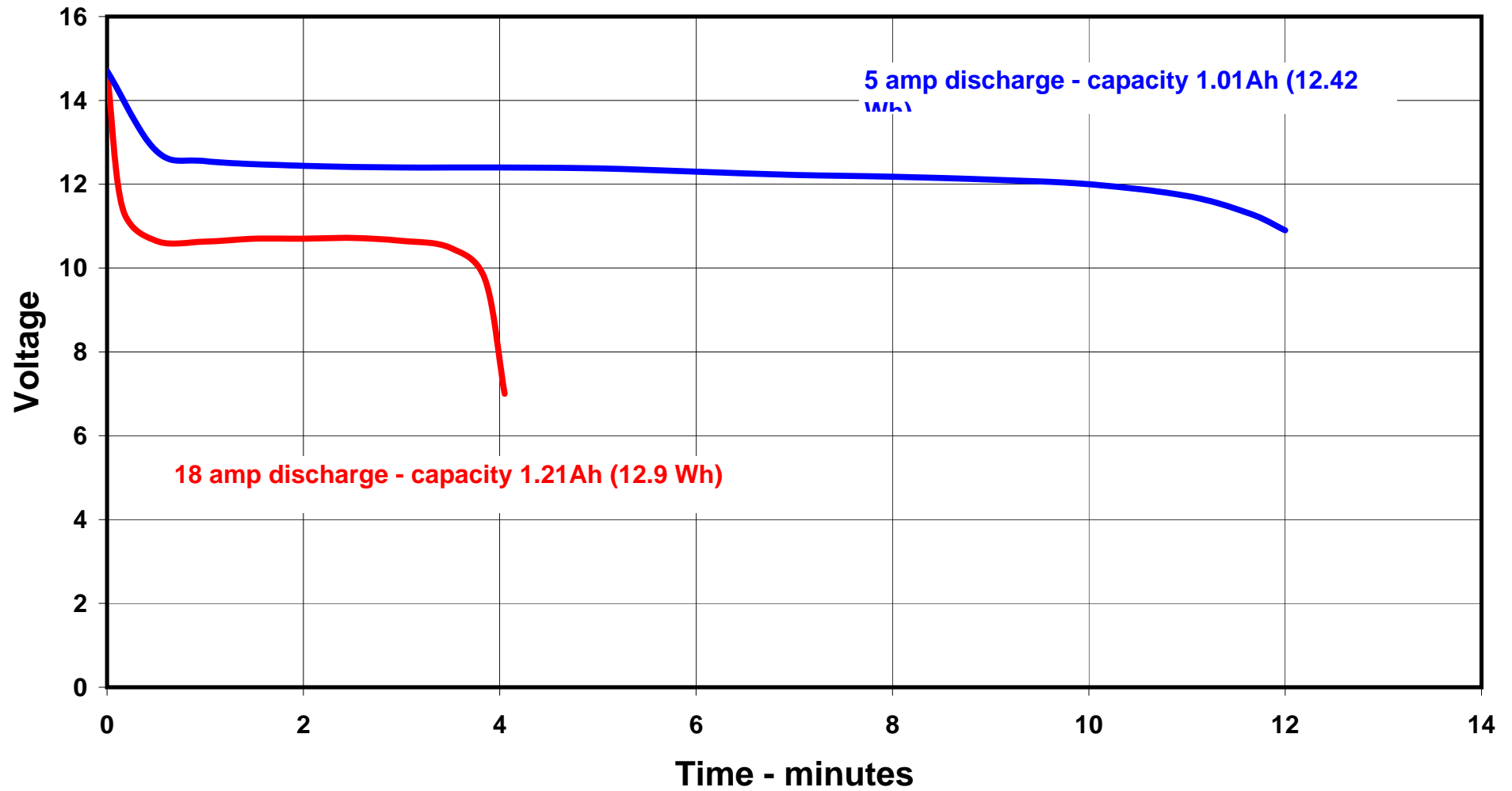
Graph 1 - 4S Saphion Discharge at 5 & 18 amps.
