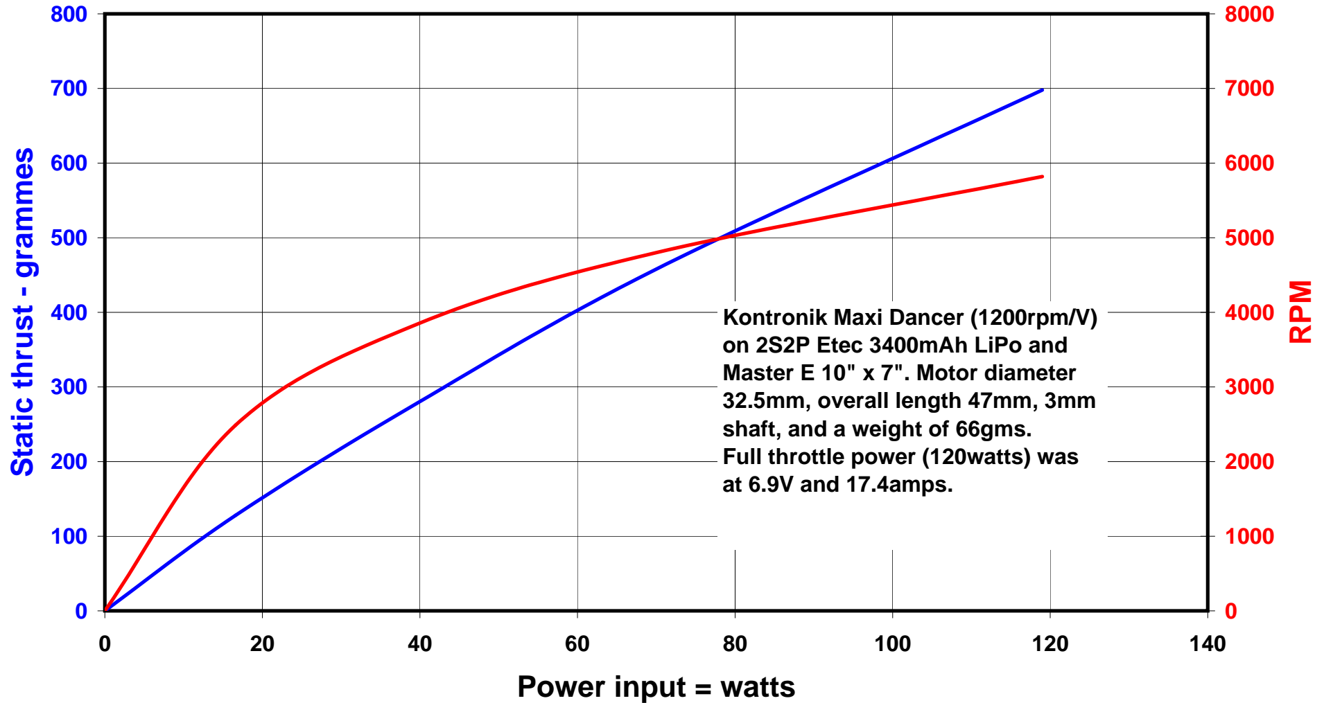
Graph 8 - Kontronik Maxi Dancer.
