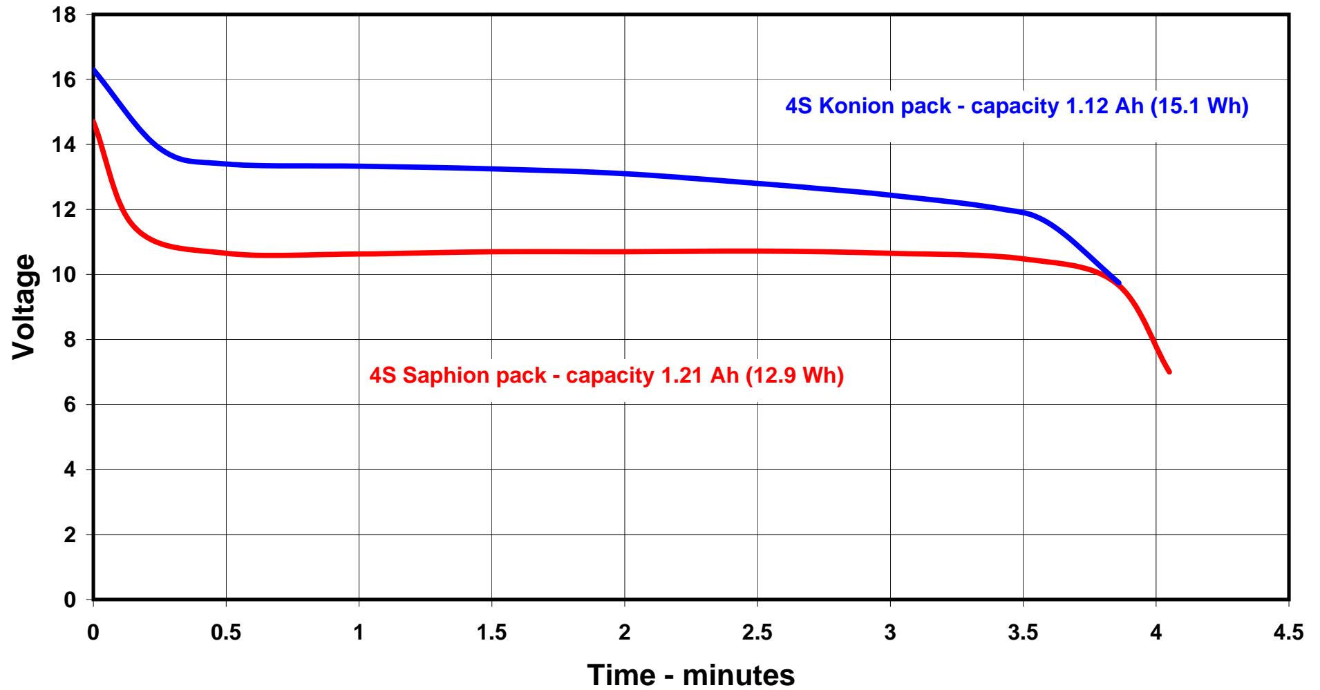
Graph 2 - Discharge at 18 amps - Konion & Saphion
