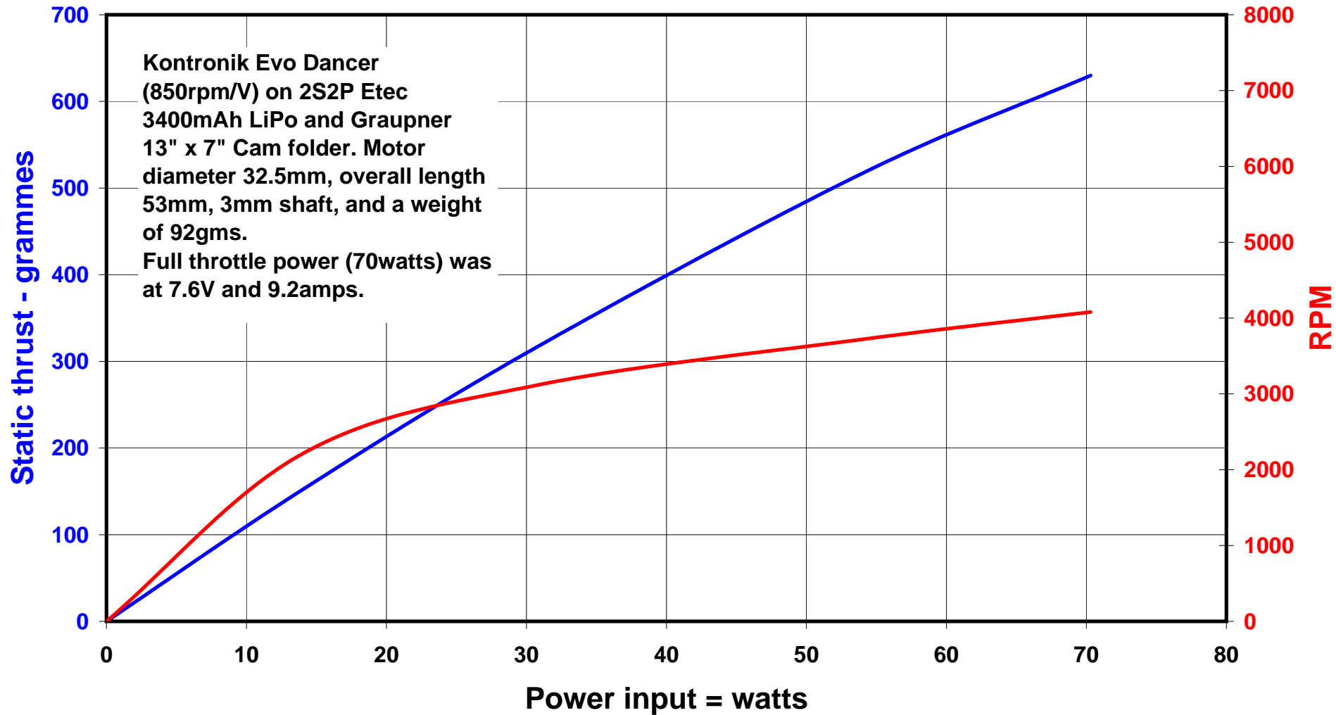
Graph 9 - Kontronik Evo Dancer.
