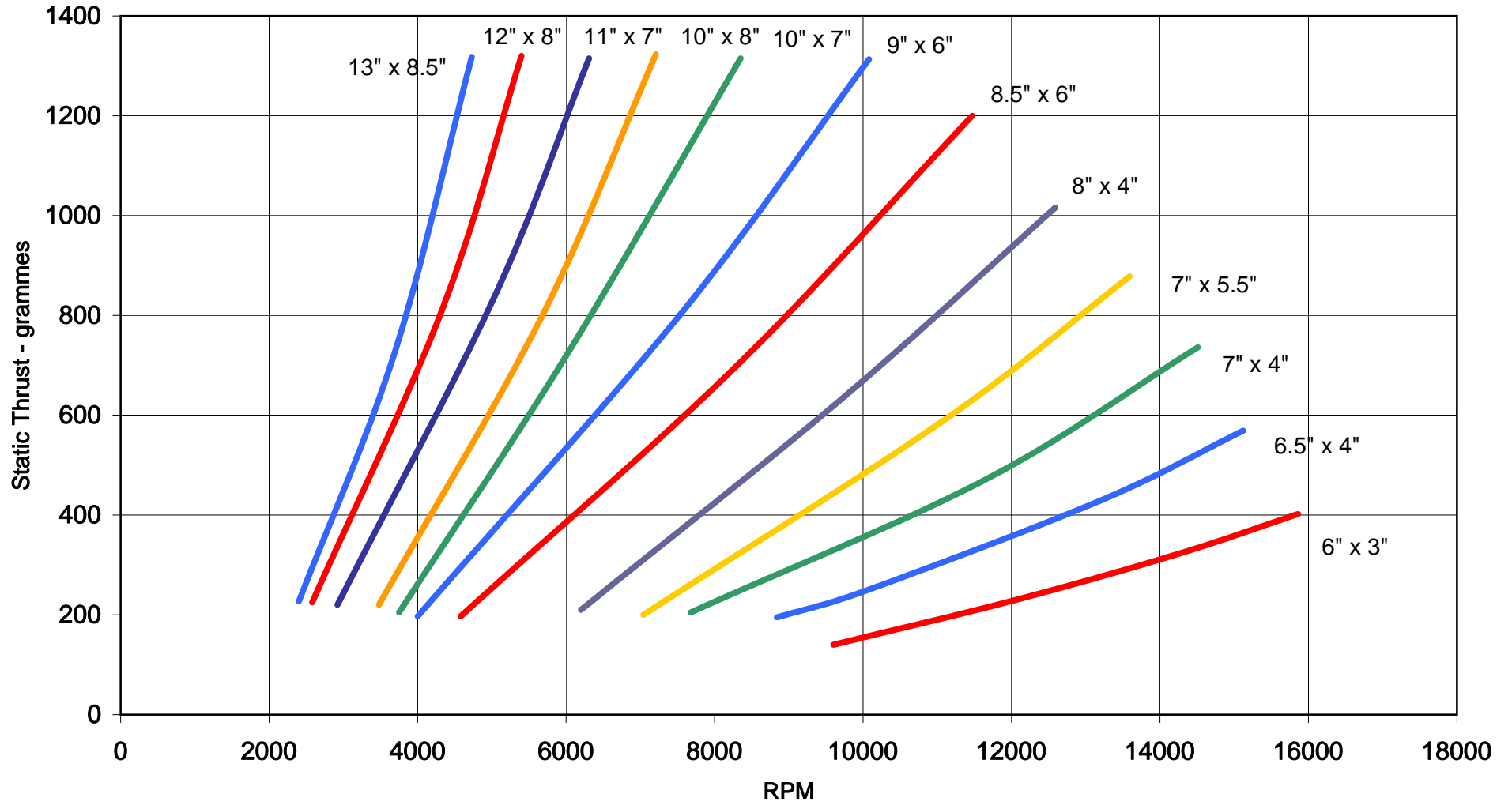
Graph 1 - Static Thrust curves for Master Electric Only Props
