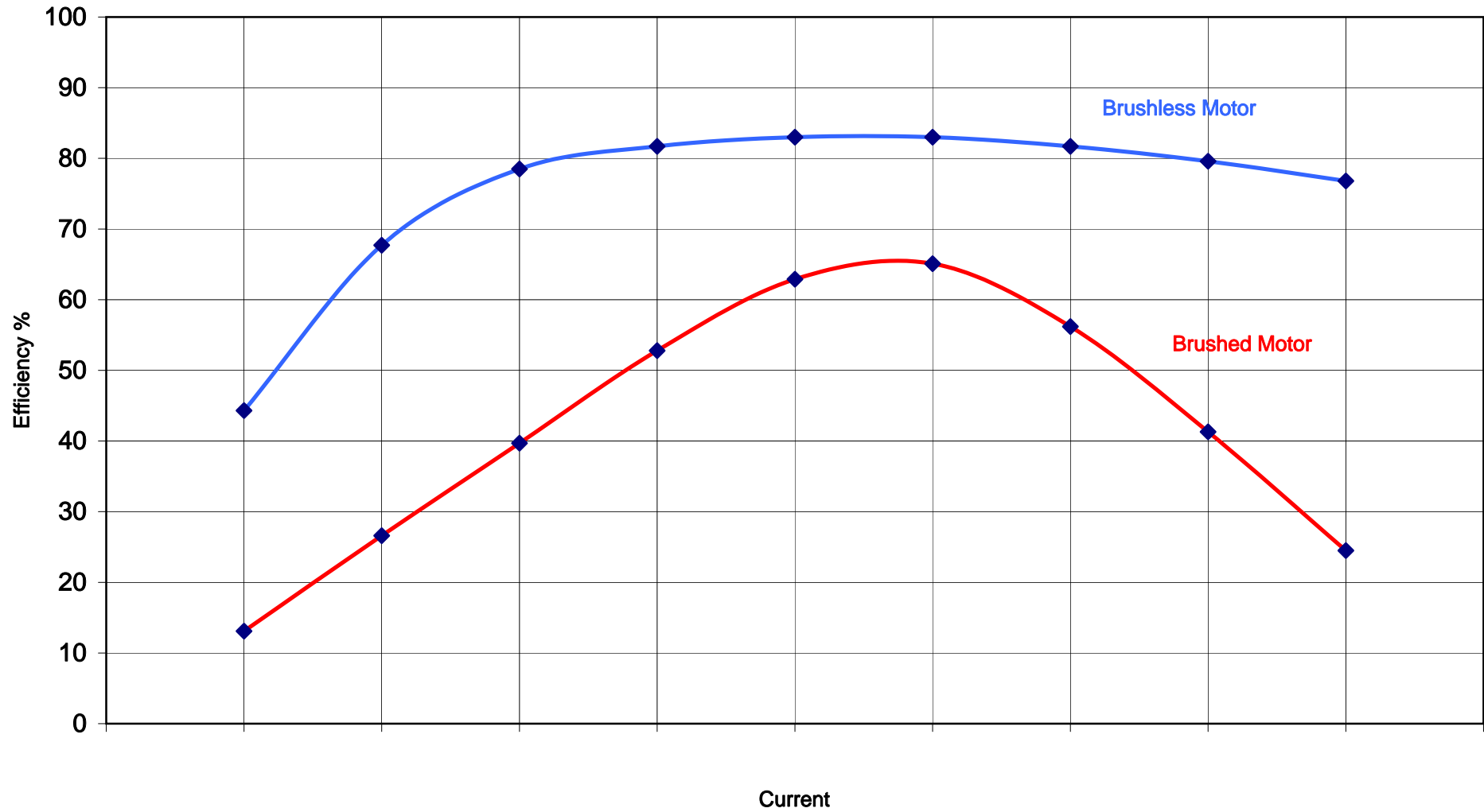
Typical efficiency curves for brushed and brushless motors.
